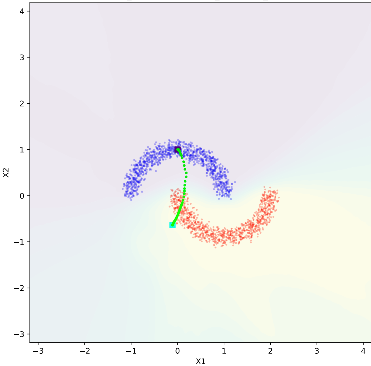
two_moon - connected_reference_point
