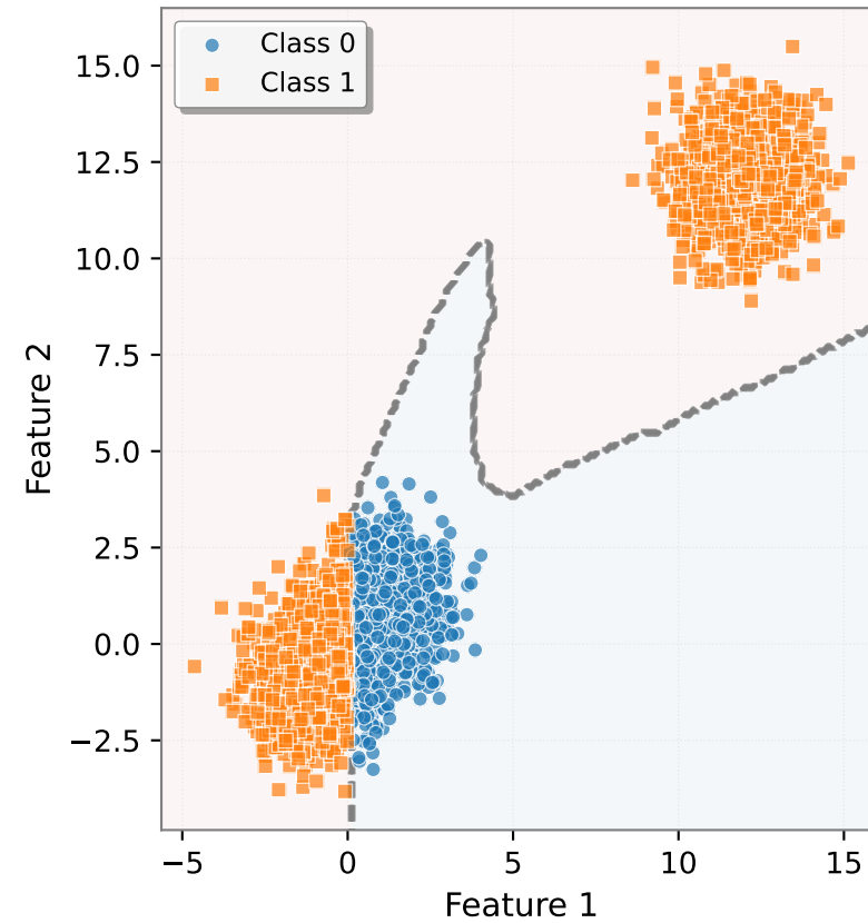
Decision Boundary: bubbles_noisy
