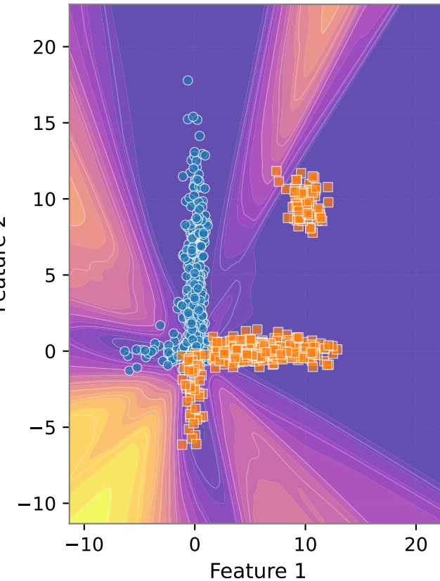
Epistemic Uncertainty (EU)
