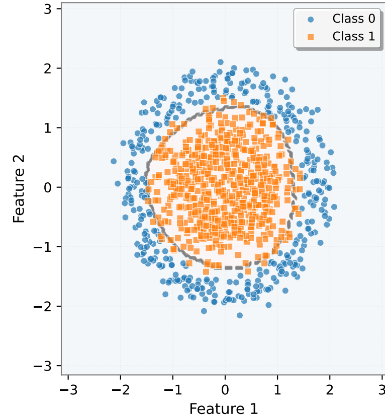
Decision Boundary: ring_dataset
