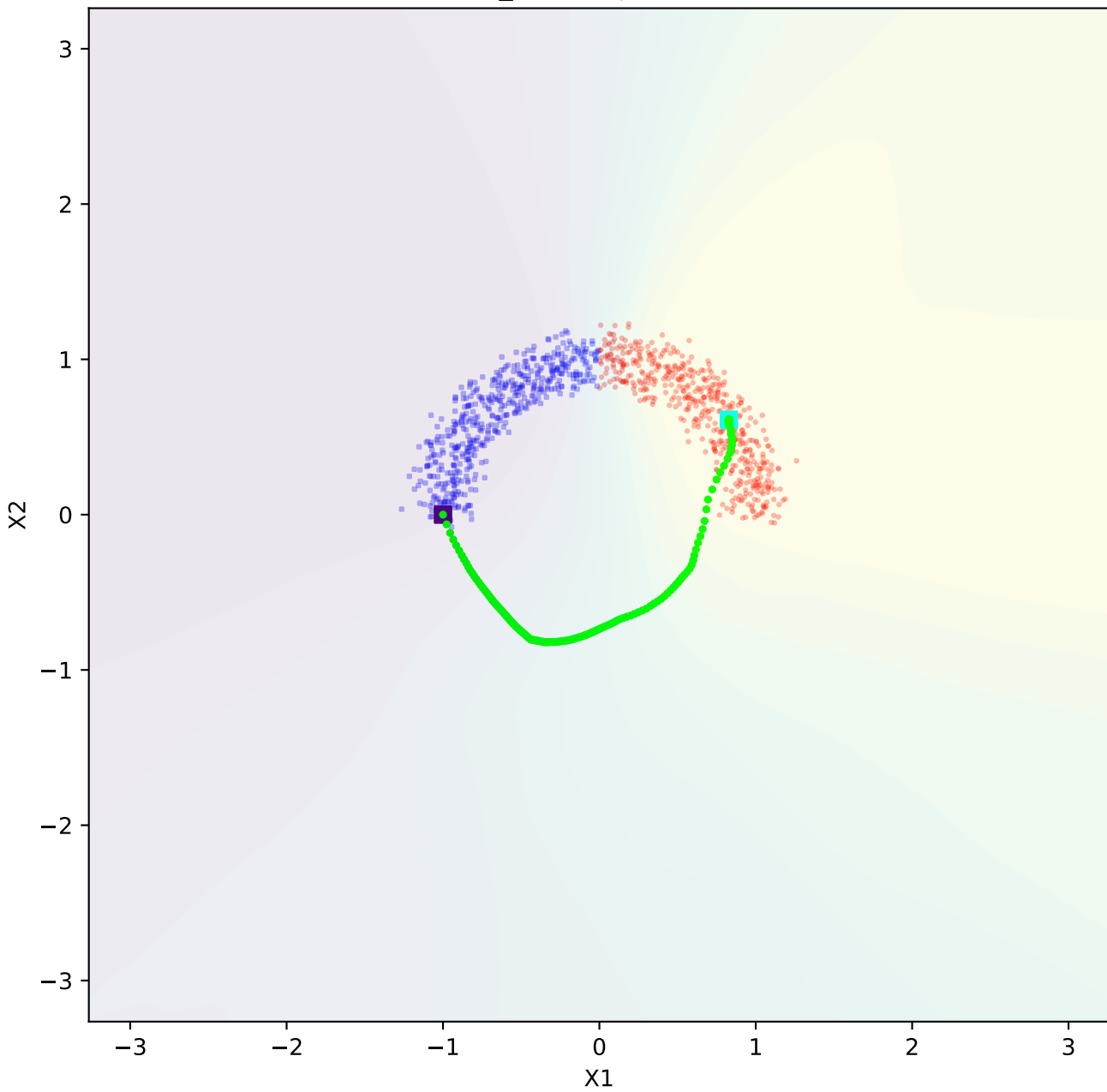
one_moon - plausible
