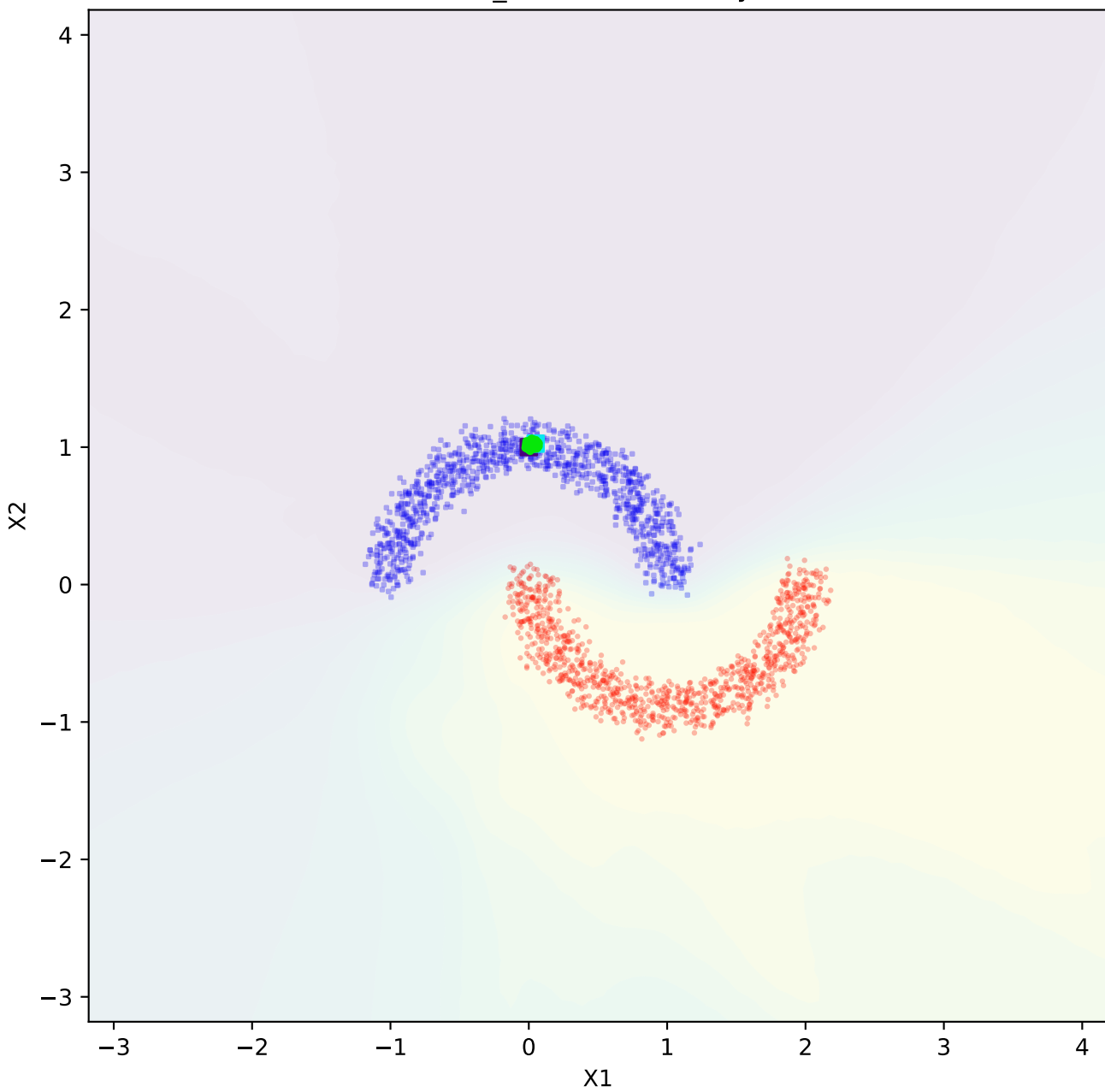
two_moon - feasibility
