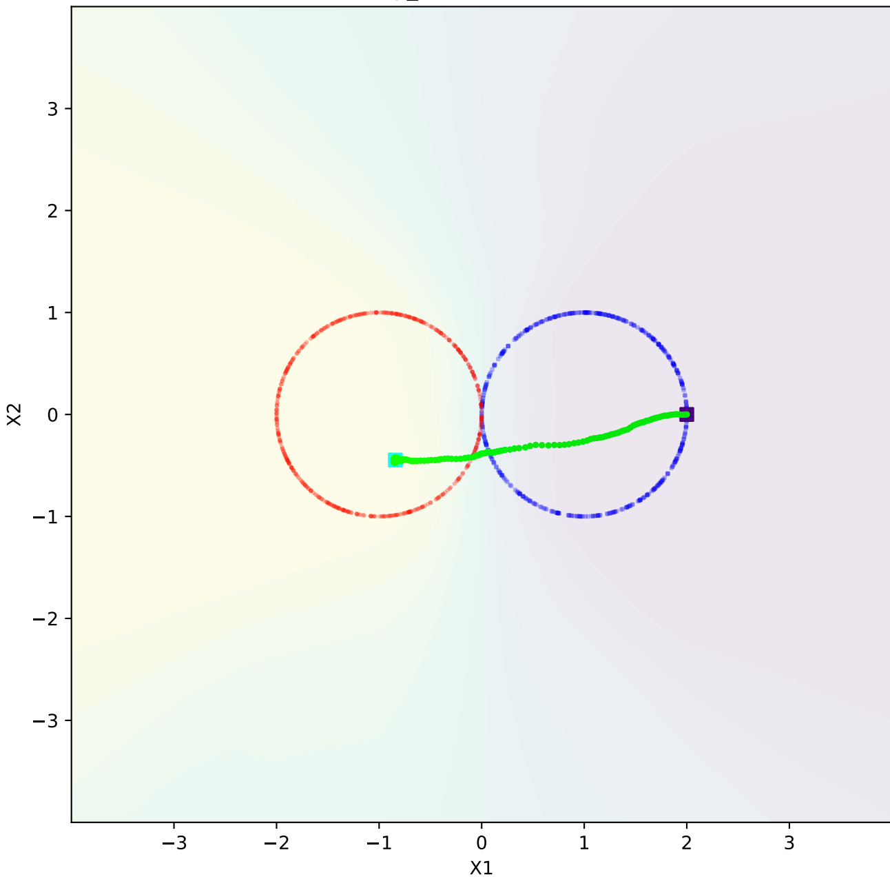
infinity_dataset - combined
