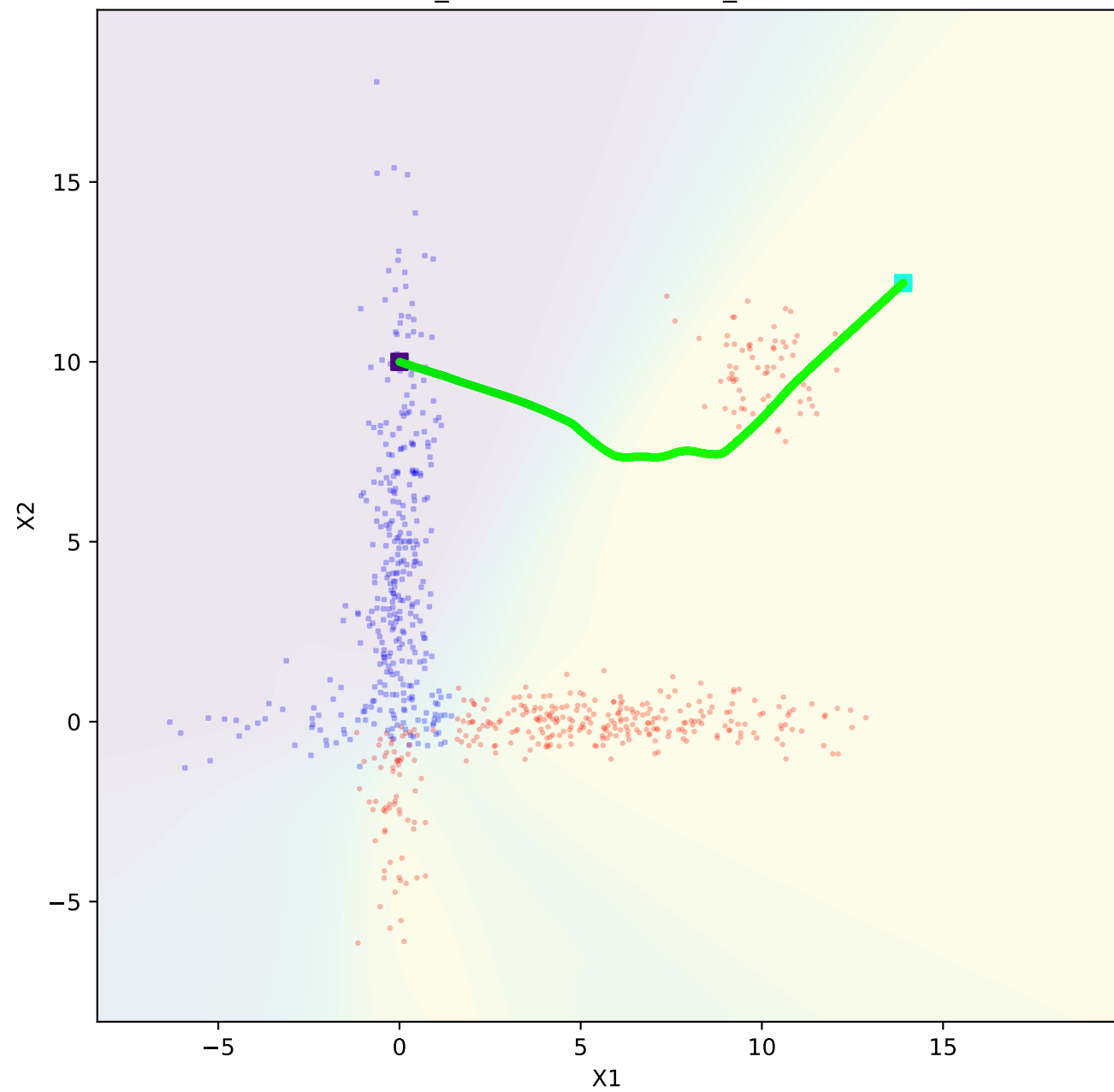
l_dataset - connected_ball
