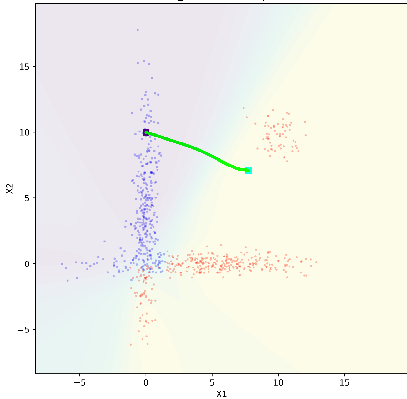
l_dataset - validity
