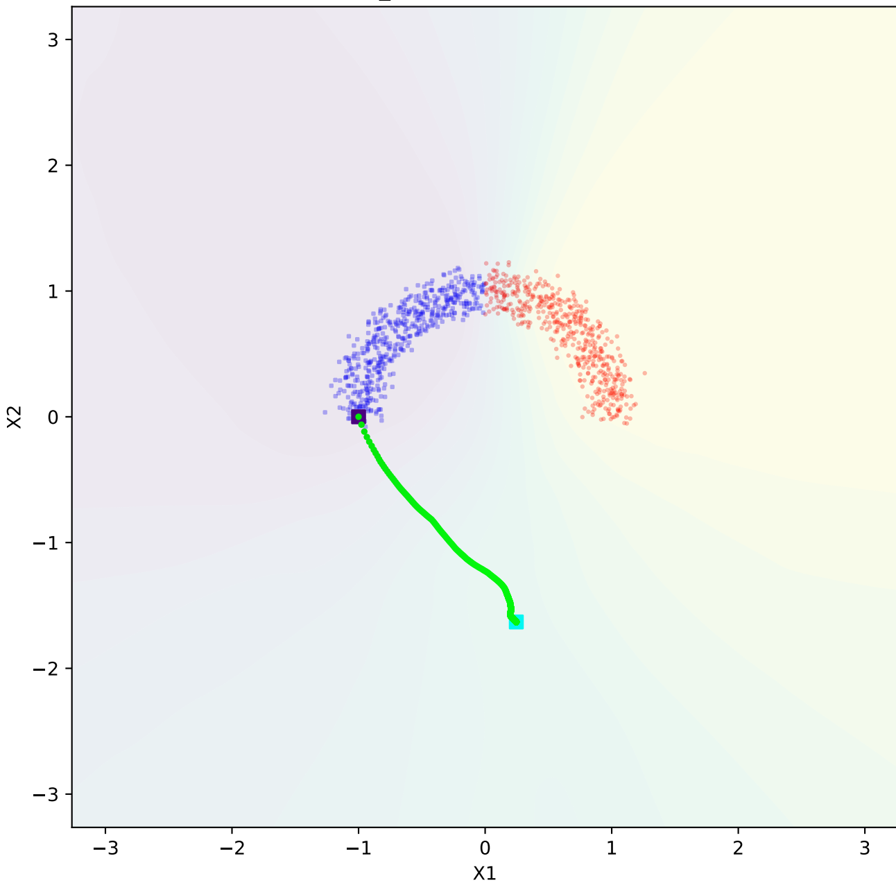
one_moon - discriminative
