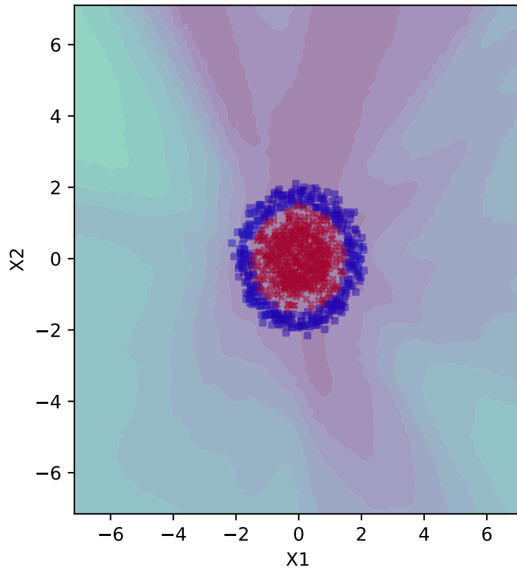
Hyper_MEAN_EU
