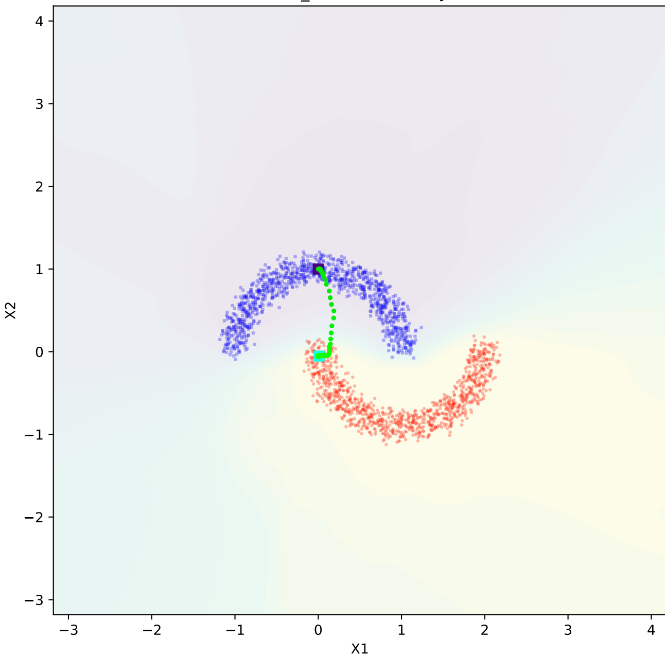
two_moon - similarity
