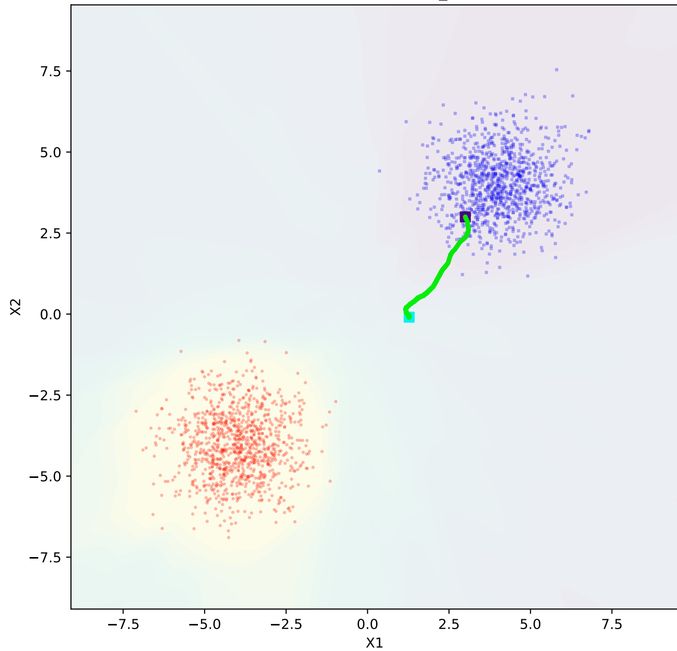
bubbles - connected_ball
