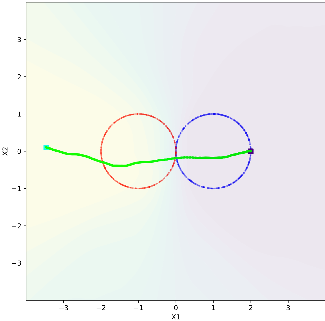
infinity_dataset - discriminative
