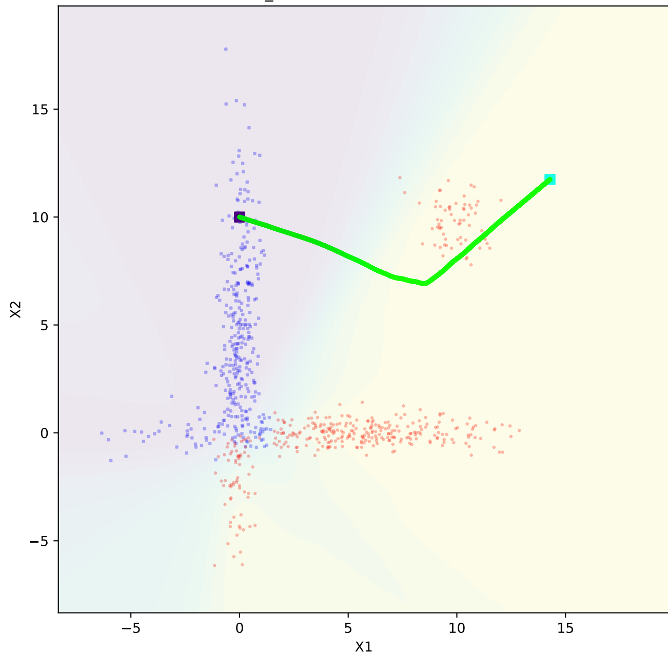
l_dataset - discriminative
