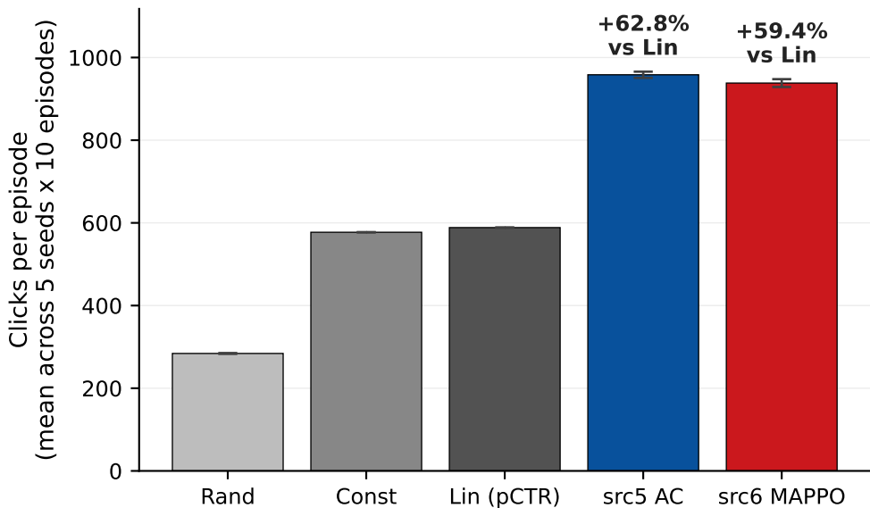
Held-out evaluation: clicks by policy
