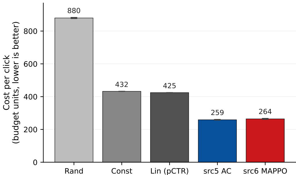
Bidding efficiency: cost per acquired click
