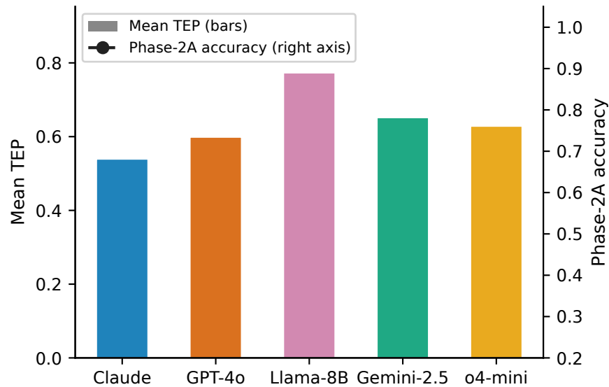
(b) Trajectory error propagation GSM, n=44; Acc_P2A not stored
