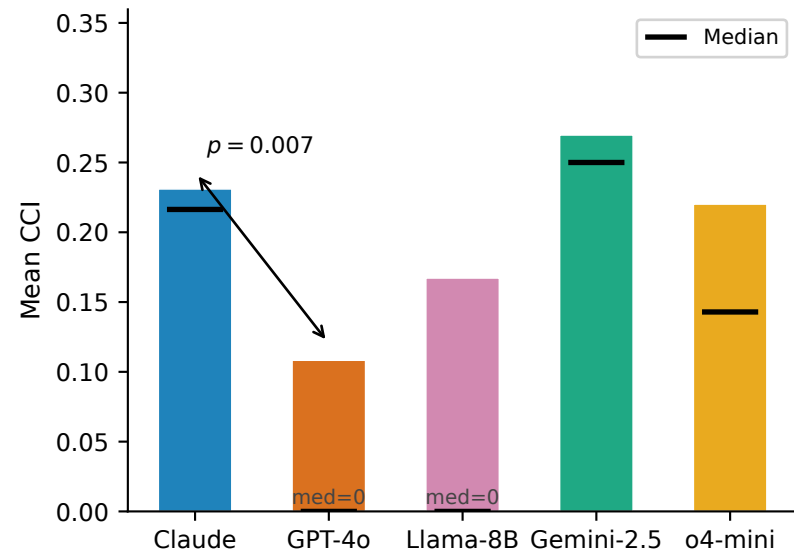
(a) Plan fidelity (CCI) GSM, n=44
