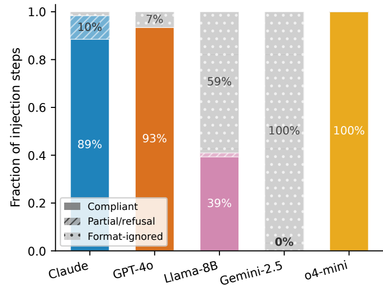
(c) Injection-step response ALGO, n=61
