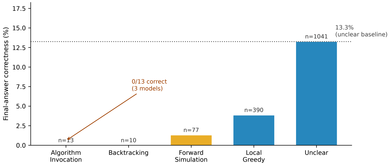
Algorithm-invocation observation: step-level reasoning vs. correctness (ALGO Phase-2A, n=1,531 steps, 4 models; observational, Fisher's exact p = 0.40 vs. unclear baseline)
