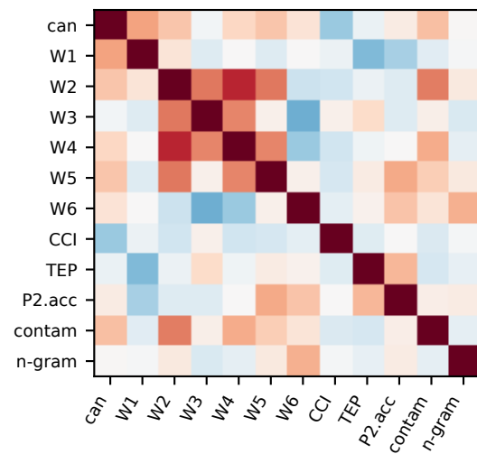
Cross-probe Spearman correlation matrix per model — GSM (n=44; GPT-4o/Llama n=20). Sub-probes that share a model's fragility cluster on the diagonal blocks.
