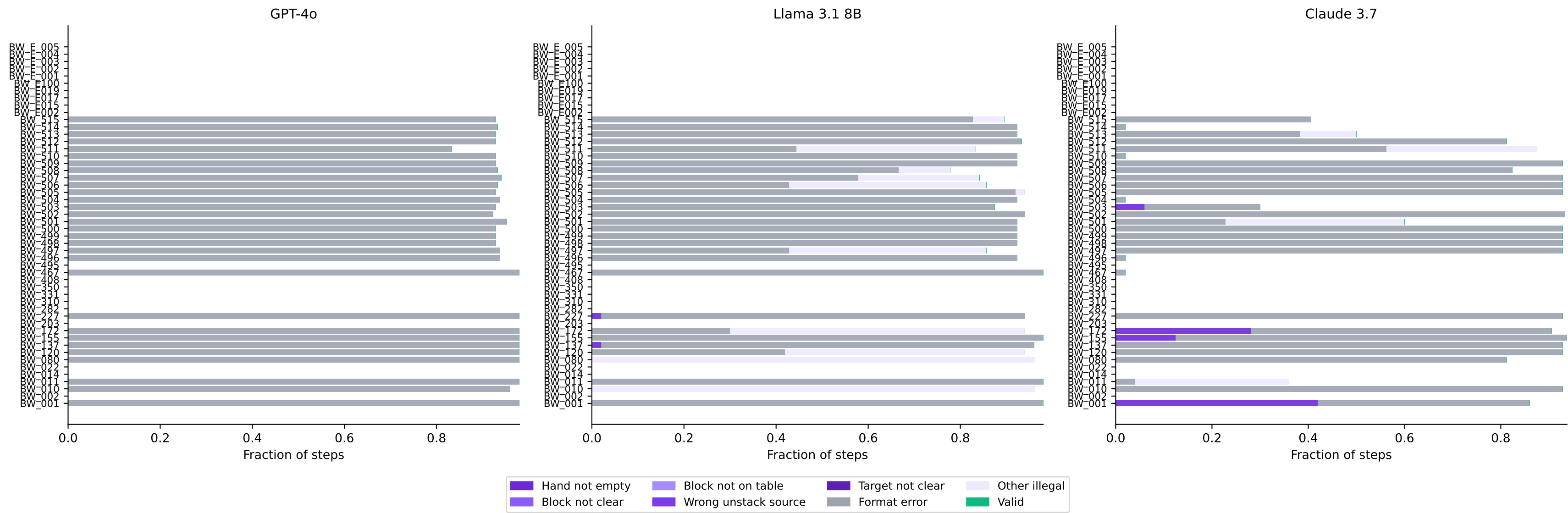
Figure 5 — Precondition Violation Profile per Problem (Probe 2: mechanistic failure breakdown)
