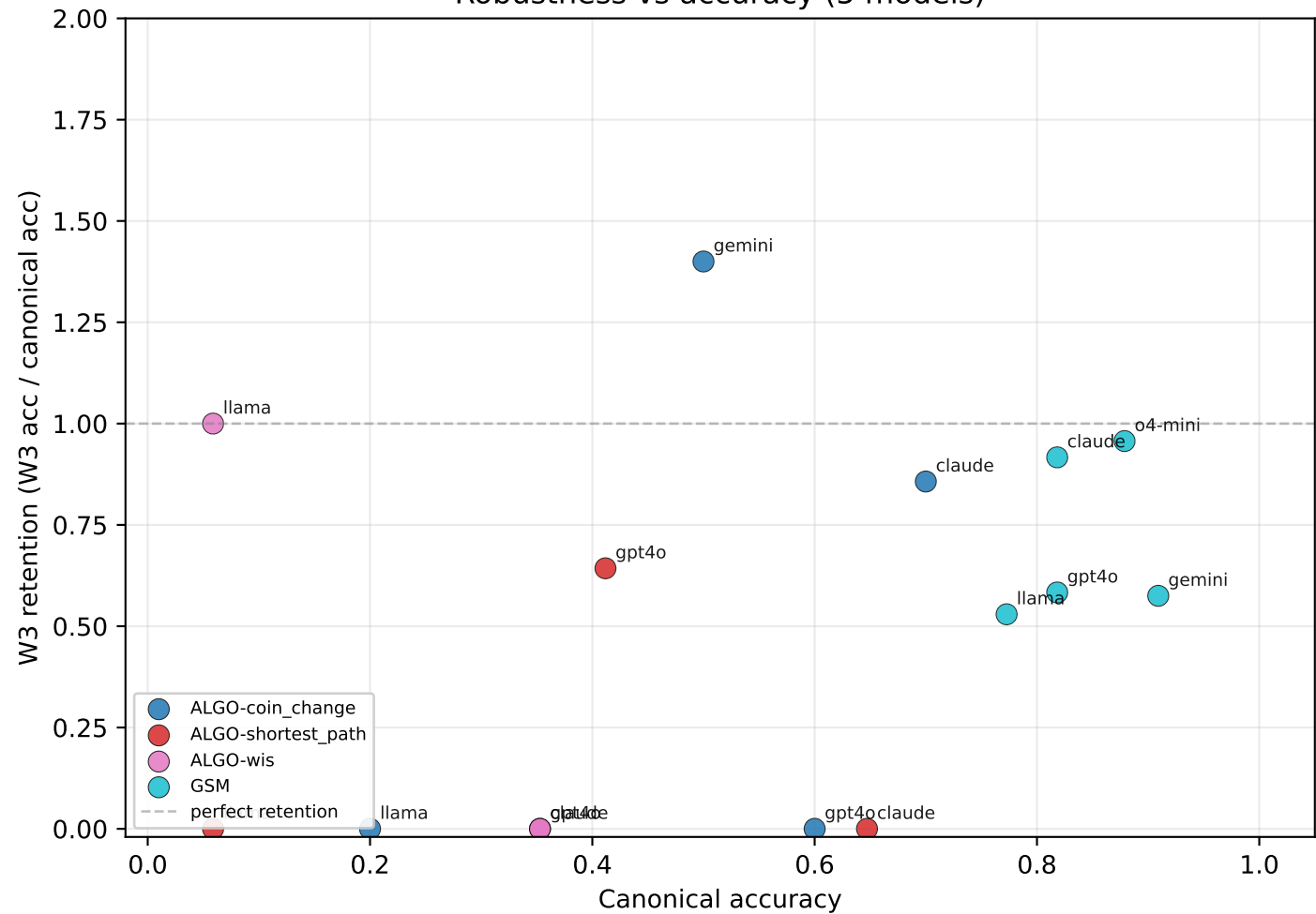
Robustness vs accuracy (5 models)
