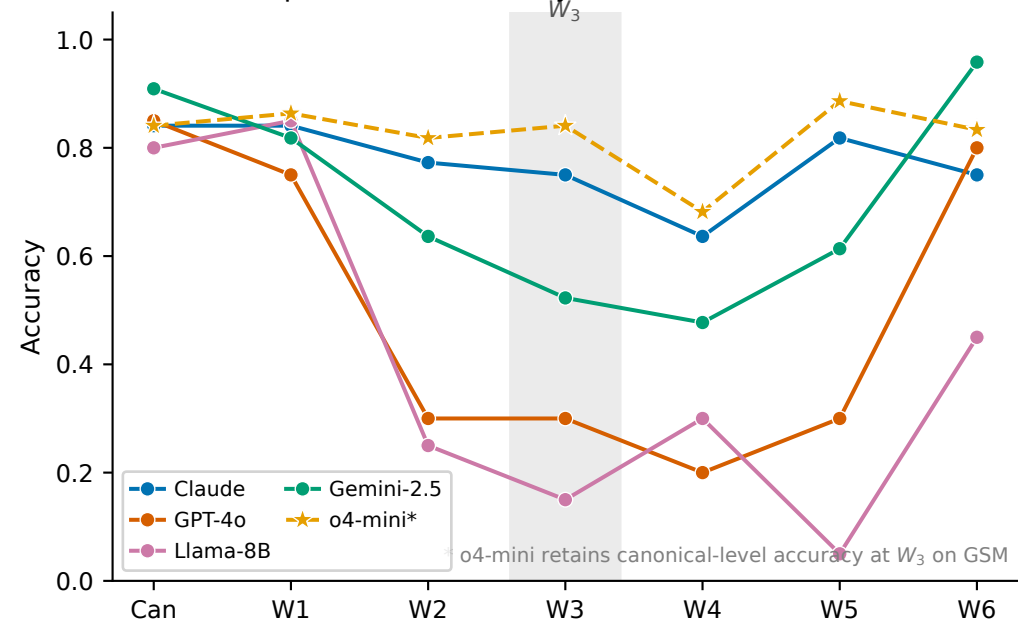
(a) GSM: per-variant accuracy (n=44; GPT-4o/Llama n=20)
