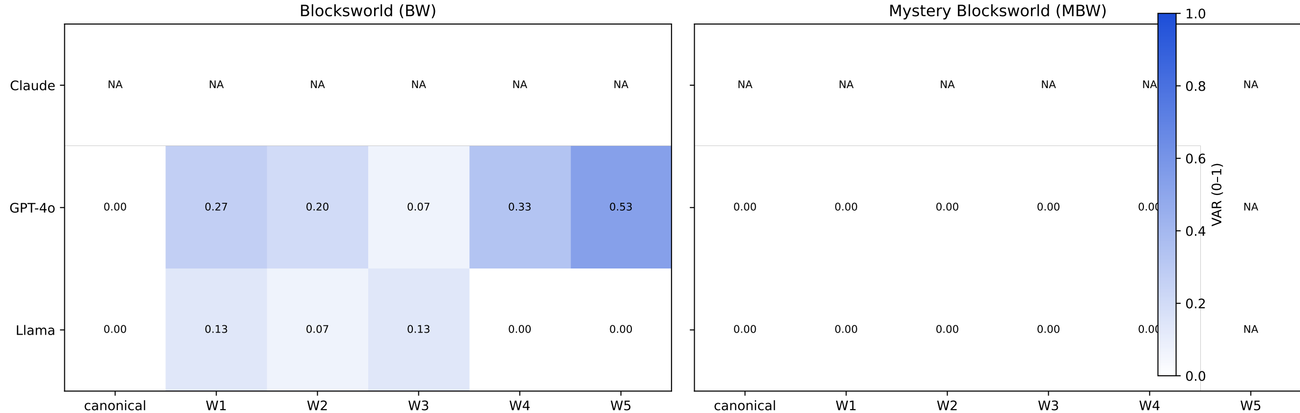
Figure 1 — Variant Accuracy Rate (VAR) Heatmap
