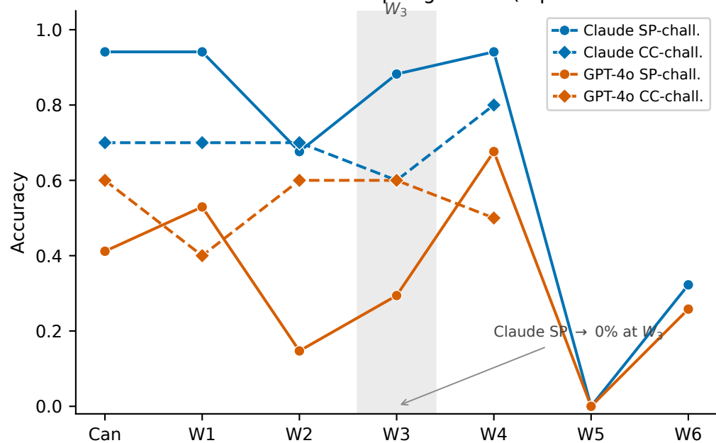
(b) Challenging ALGO subtypes (Claude vs. GPT-4o) ALGO effective n=51 after collapsing clones (reported on 110 IDs)
