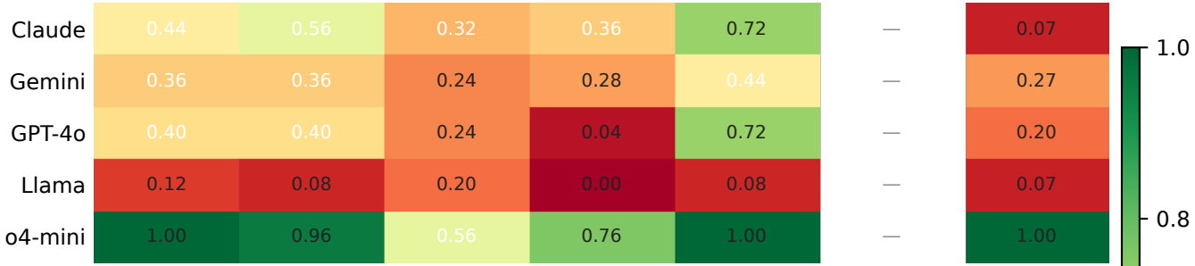
Coin change (greedy)
