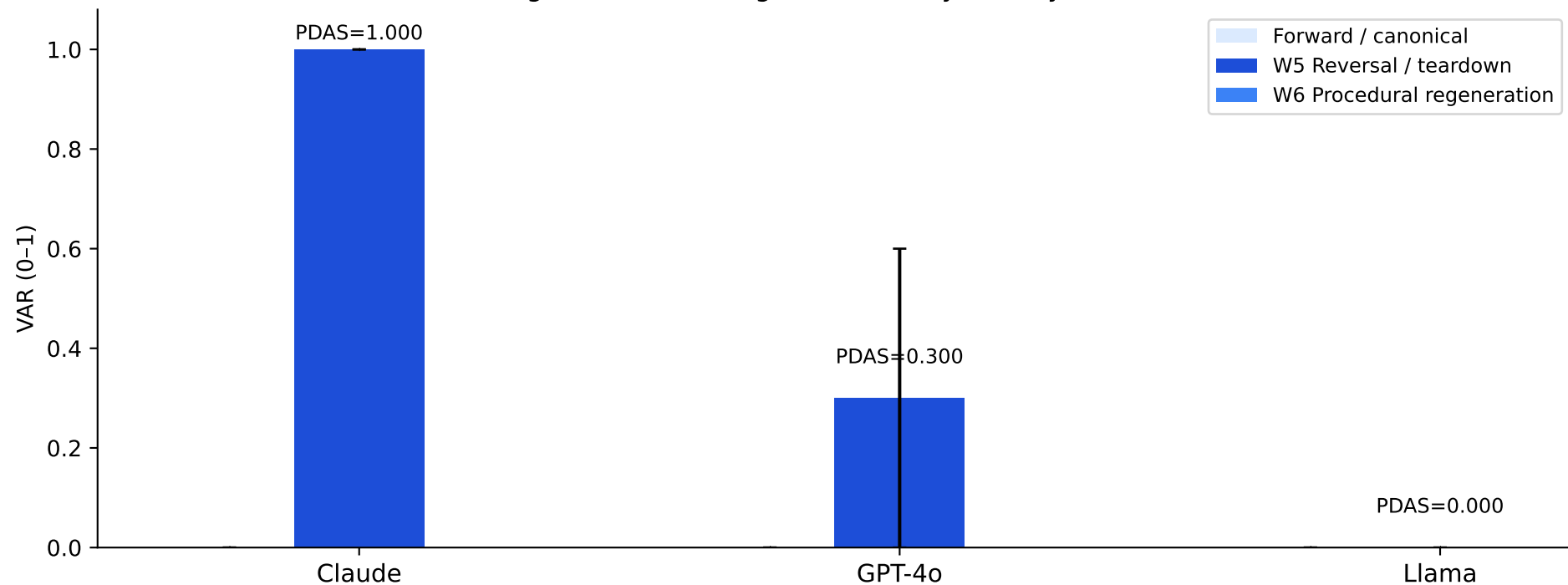
Figure 2 — Planning Direction Asymmetry (PDAS)
