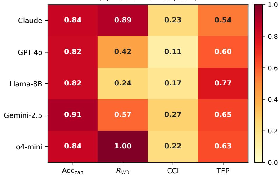
(a) Macro metrics (GSM)
