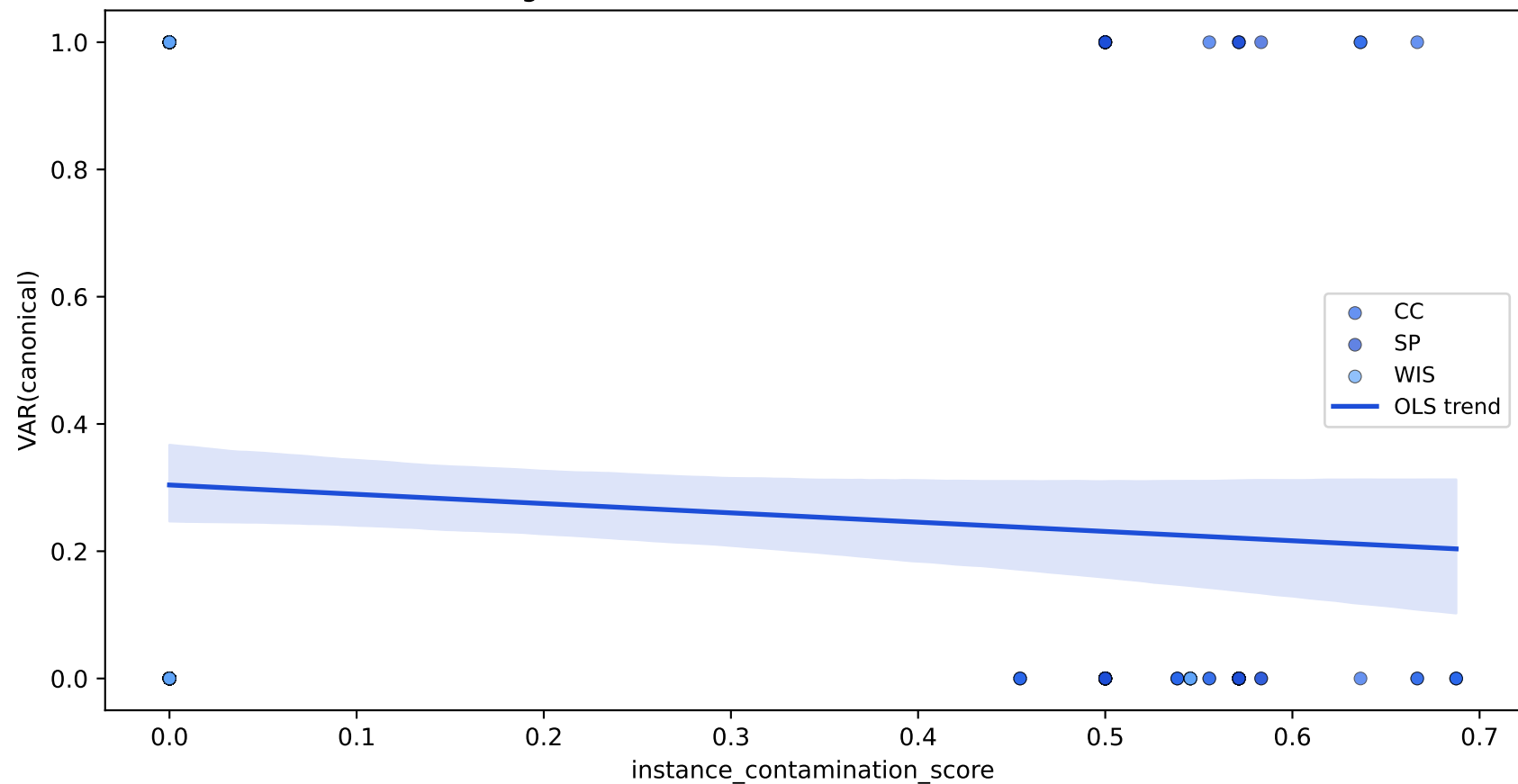
Figure 4 — Contamination vs canonical VAR
