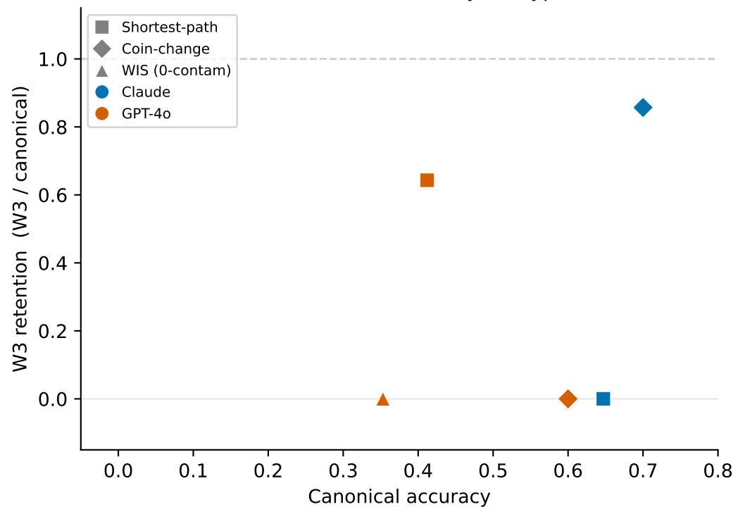
(b) Adversarial ALGO by subtype
