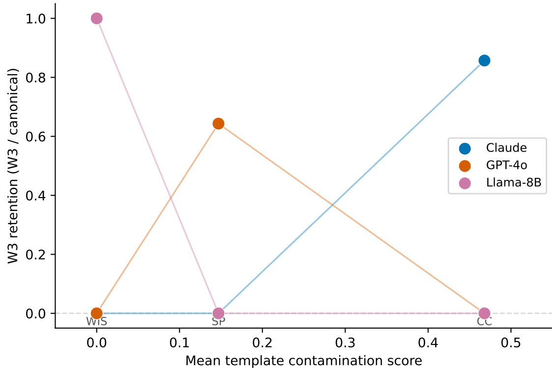
(b) W3 retention vs template contamination (within-family control)
