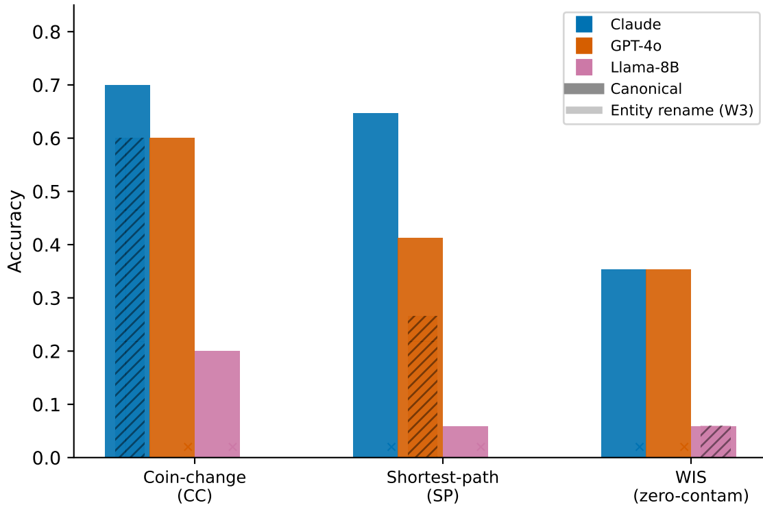
(a) Adversarial accuracy under canonical and entity rename (W3)
