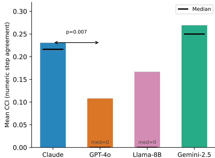
(a) Plan-Execution Coupling (CCI)
