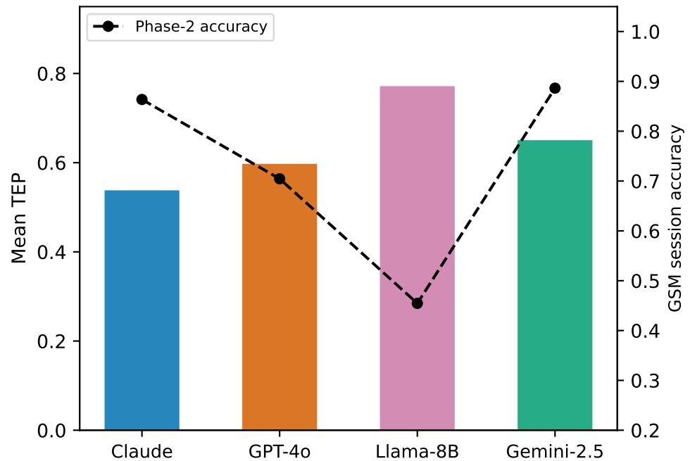
(b) Trajectory Error Propagation (TEP)
