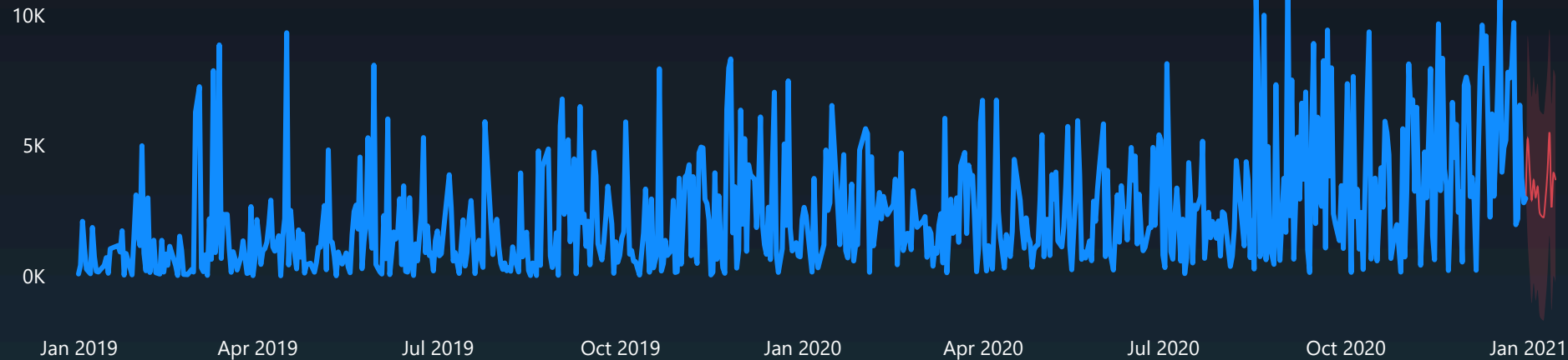
Forecasting Sales by Order Date
