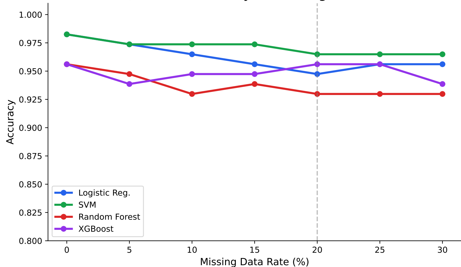
RQ1: Model Accuracy vs. Missing Data Rate
