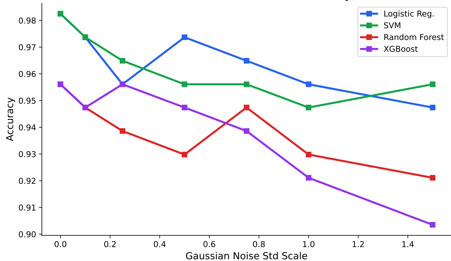
RQ2: Robustness to Gaussian Noise Injection
