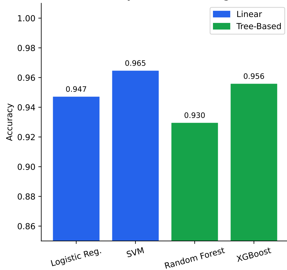
RQ4: Accuracy at 20% Data Degradation
