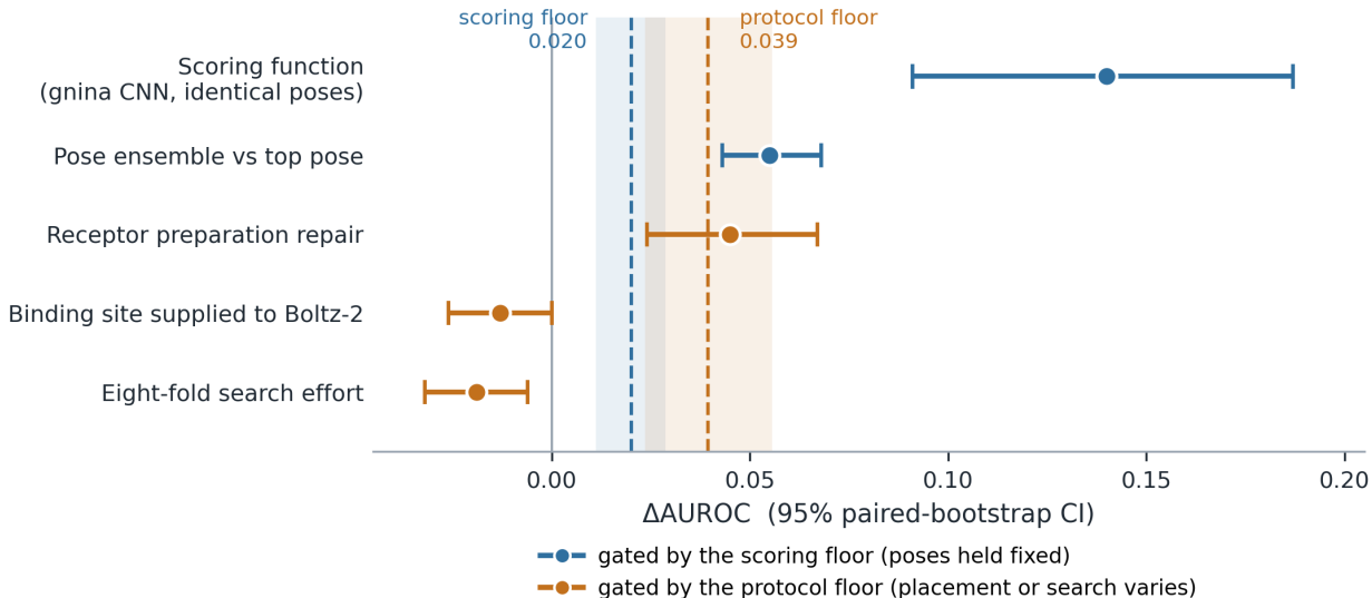
Figure 1: Five of the six interventions against the two measured resolution limits. The pose-source arm is omitted because it is not evaluable on this panel (§3.2); plotting a void estimate would misrepresent it. Points are \Delta AUROC with 95% paired-bootstrap intervals; dashed lines are the two floors from §3.1 with their own bootstrap intervals shaded. Each intervention is coloured by the floor that applies to it — the scoring floor where poses were held fixed, the protocol floor where placement or search was allowed to vary. The two floor intervals overlap between 0.024 and 0.029. Note that the eight-fold search-effort comparison is the measurement that defines the protocol floor, so its effect cannot exceed it by construction.
