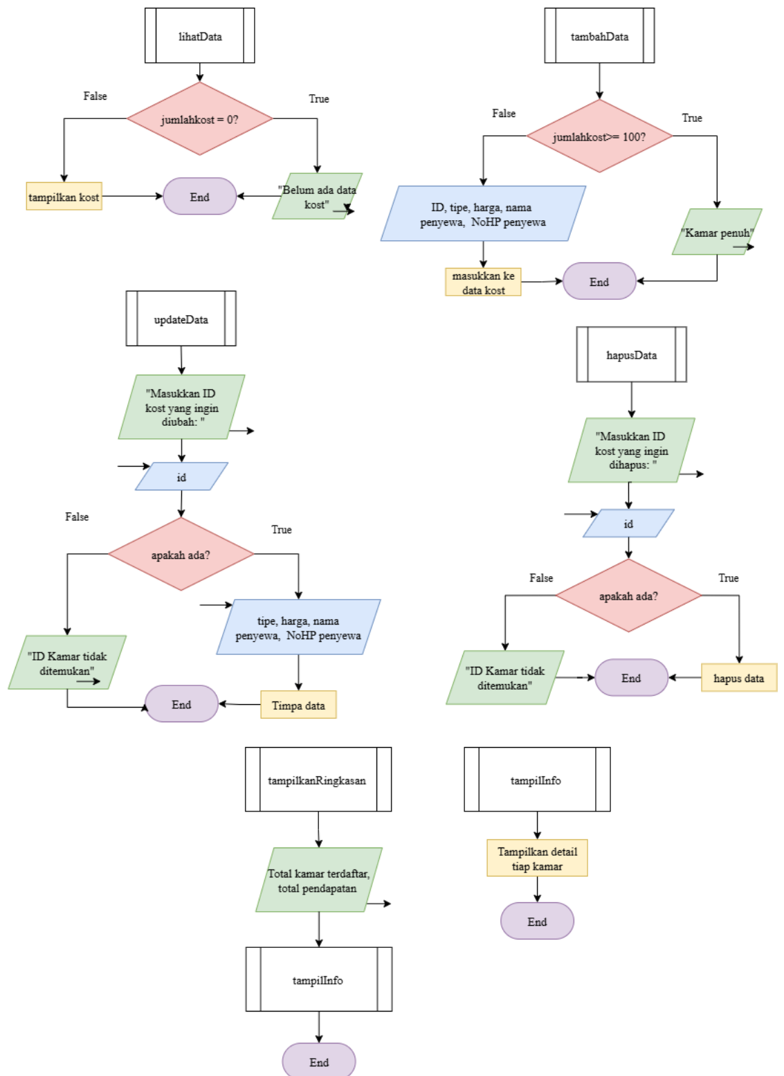
Gambar 1. 3 Flowchart CRUD
