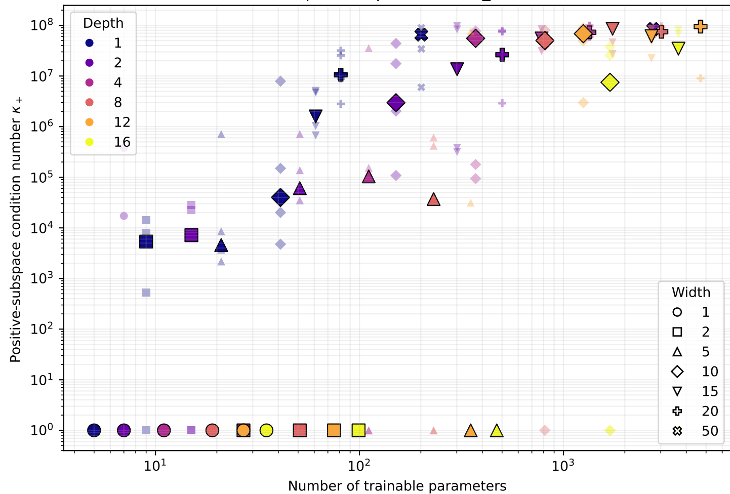
Final conditioning versus parameter count (step 1000) relu | Corner | Poisson.Ritz_Loss
