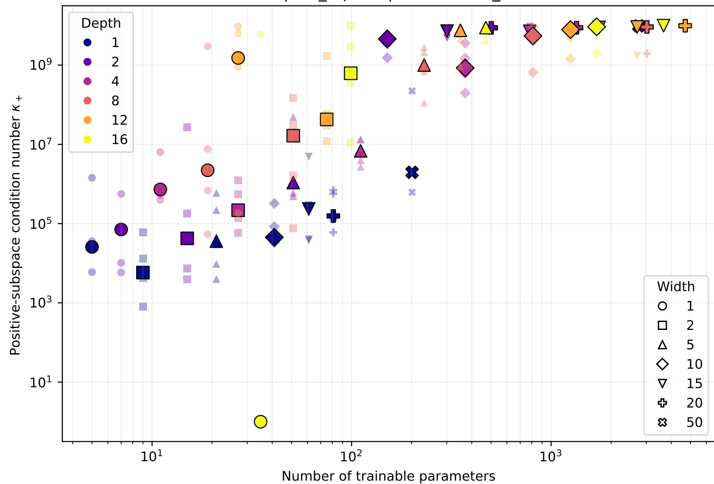
Final conditioning versus parameter count (step 1000)
