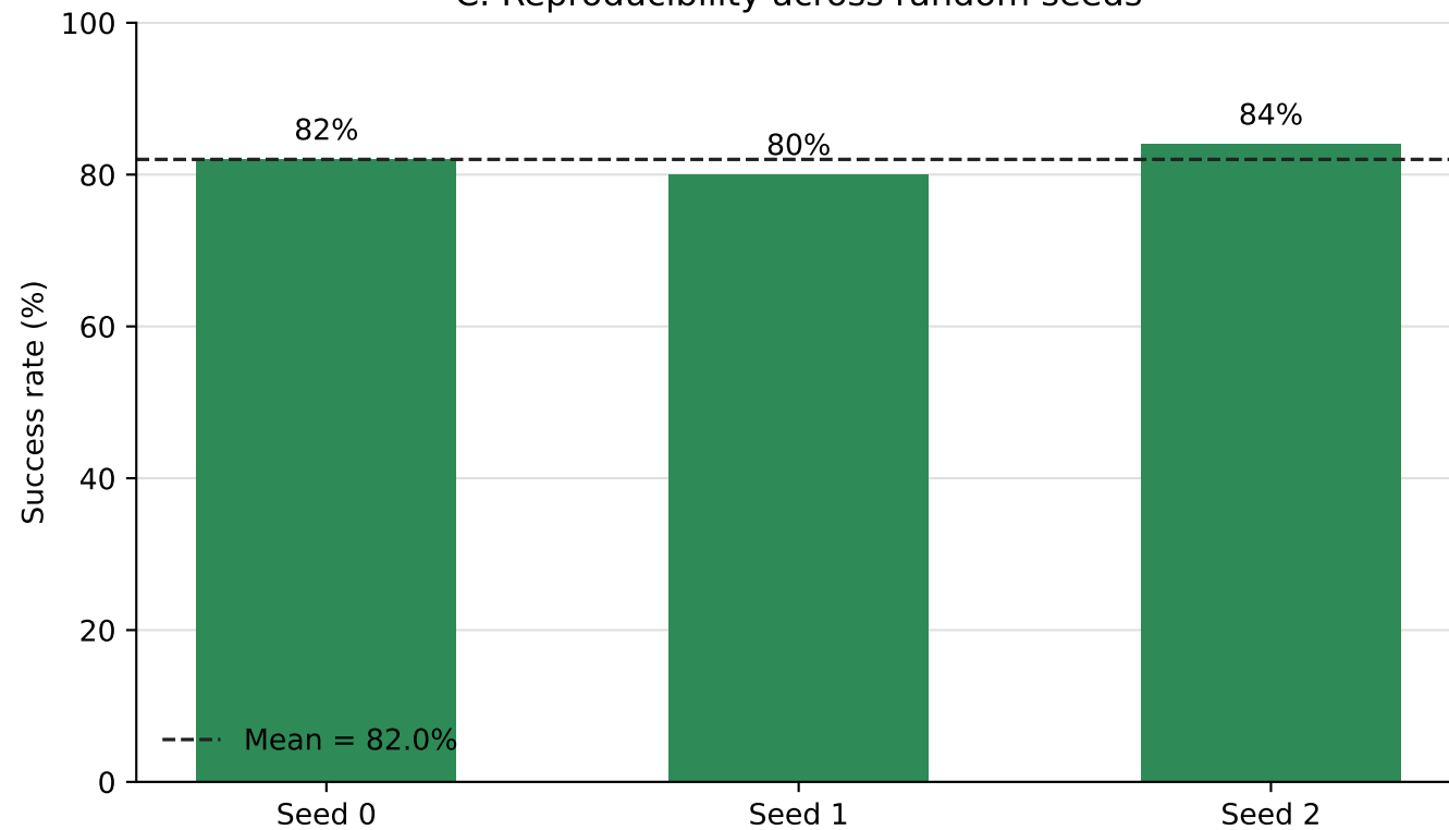
C. Reproducibility across random seeds
