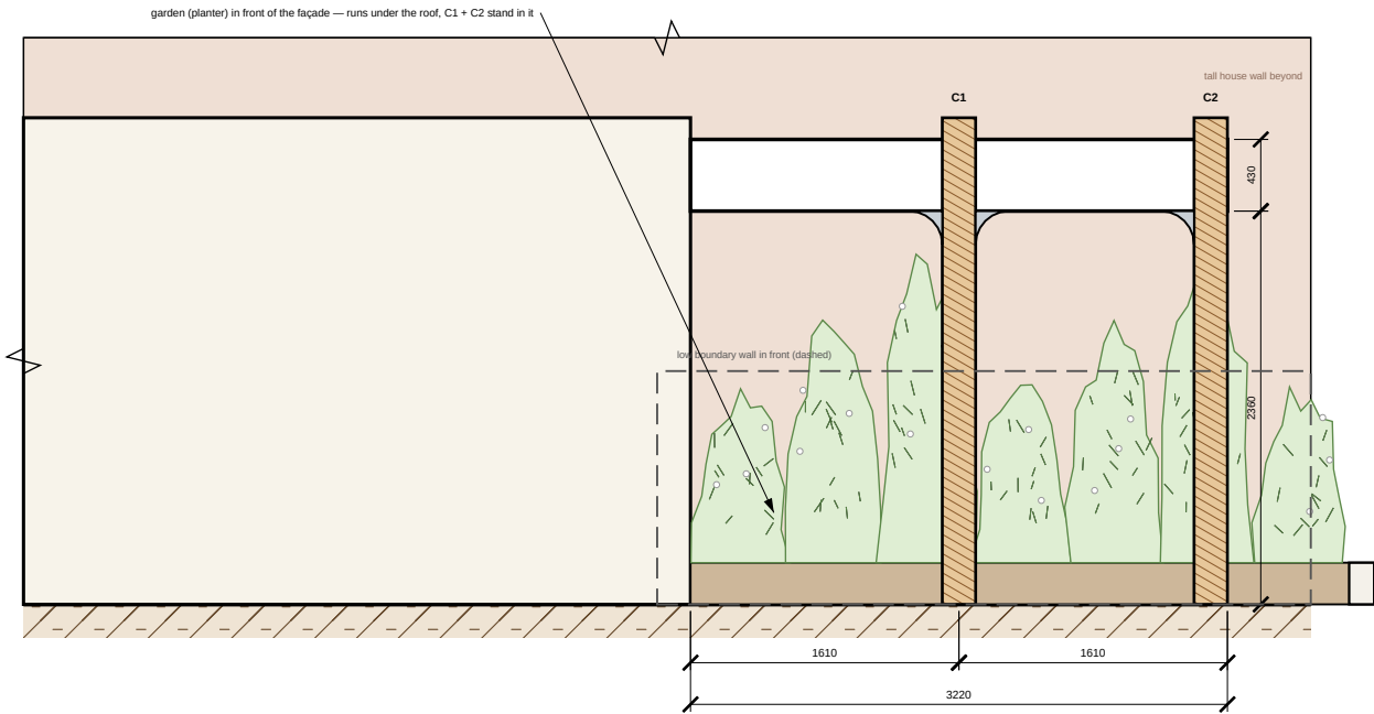
2/V2-02 PLANTS-SIDE ELEVATION — C1 + C2 — 1:50
