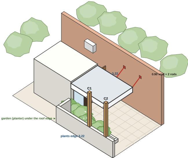
3/V2-01 3D — BIRD'S EYE (from the plants side, over the low wall)
