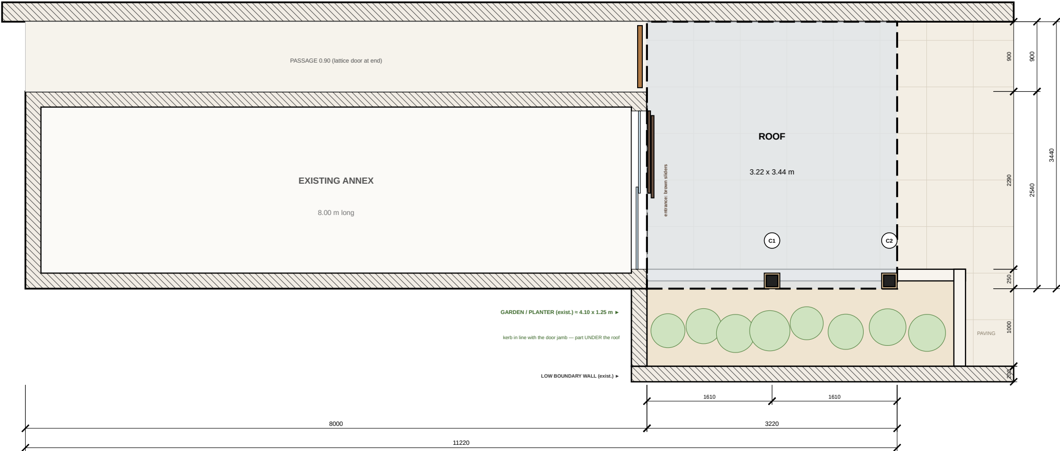
1 TOP VIEW — ANNEX, GARDEN & ROOF V1-01
