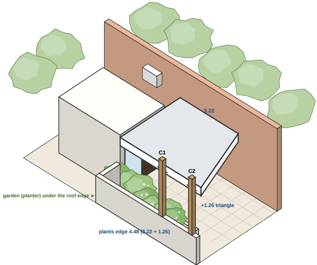
3/V1T-01 3D — BIRD'S EYE (from the plants side, over the low wall)
