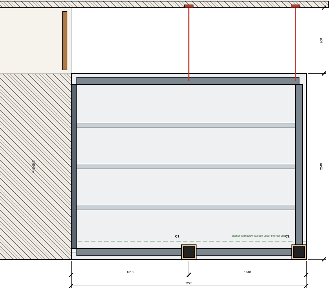
1 TOP VIEW — ANNEX, GARDEN & ROOF
