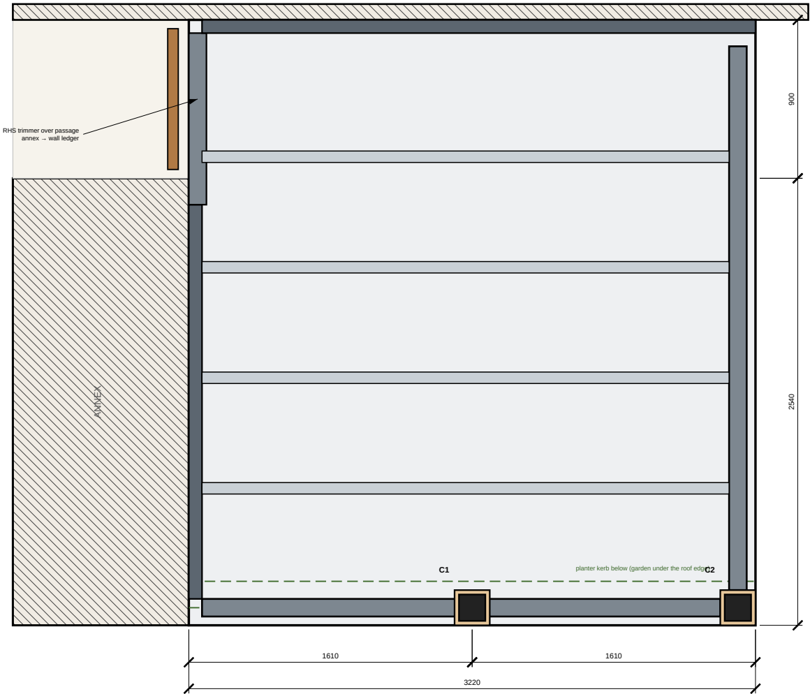
1 TOP VIEW — ANNEX, GARDEN & ROOF V1-01
