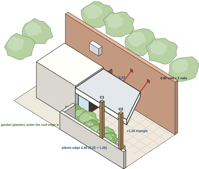
3/V2T-01 3D — BIRD'S EYE (from the plants side, over the low wall)
