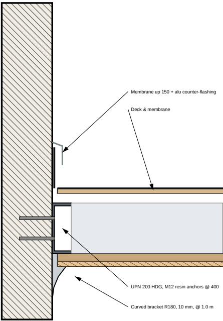
D2 COLUMN / ROOF JUNCTION (plants side) — 1:10
