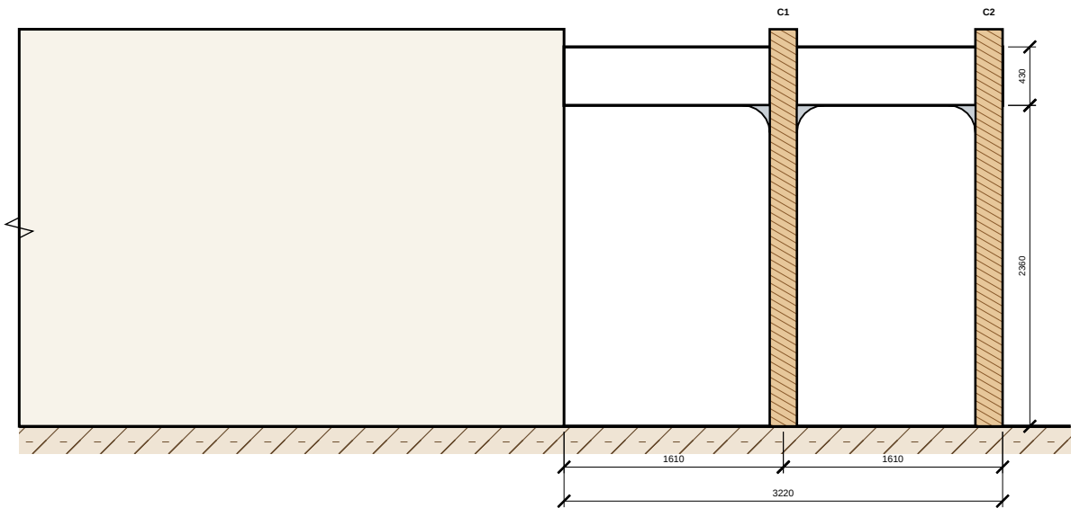
2/V2-02 PLANTS-SIDE ELEVATION — C1 + C2 (as client sketch) — 1:50
