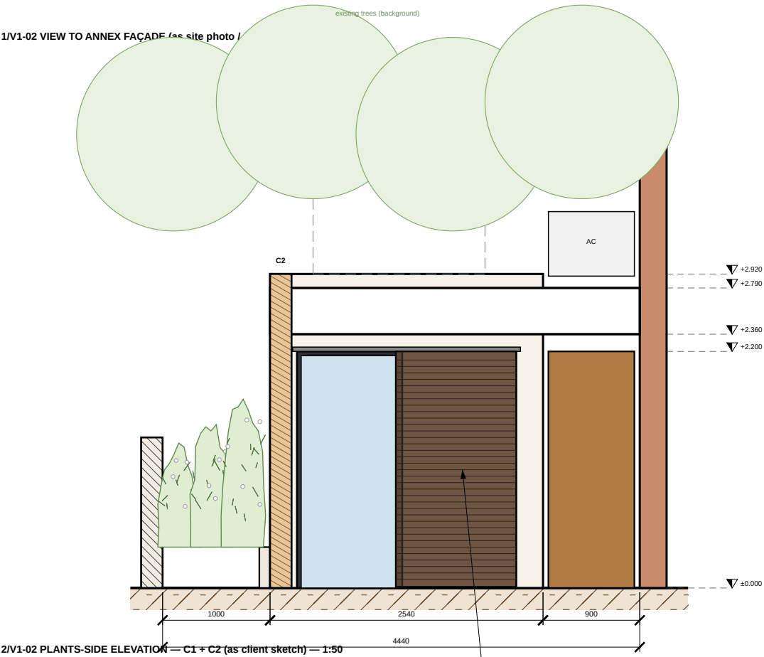
2/V1-02 PLANTS-SIDE ELEVATION — C1 + C2 (as client sketch) — 1:50
