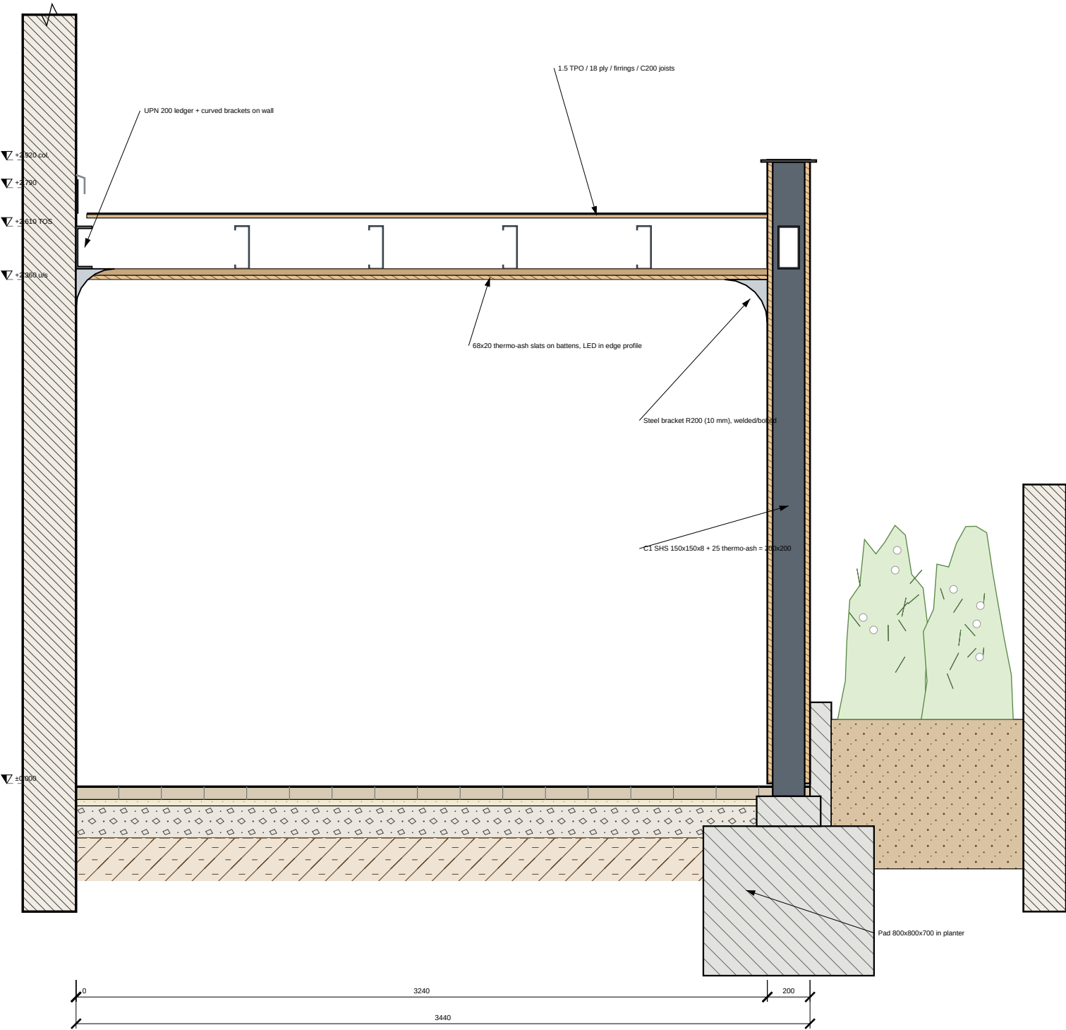
D2 COLUMN / ROOF JUNCTION (plants side) — 1:10
