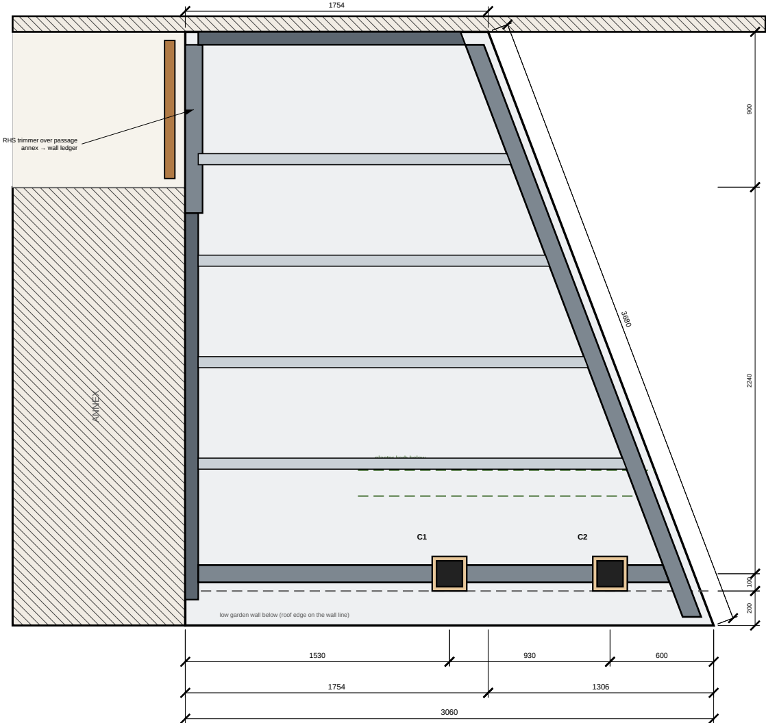
1 TOP VIEW — ANNEX, GARDEN & ROOF V1T-01
