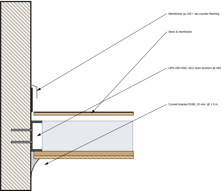
D2 COLUMN / ROOF JUNCTION (plants side) — 1:15
