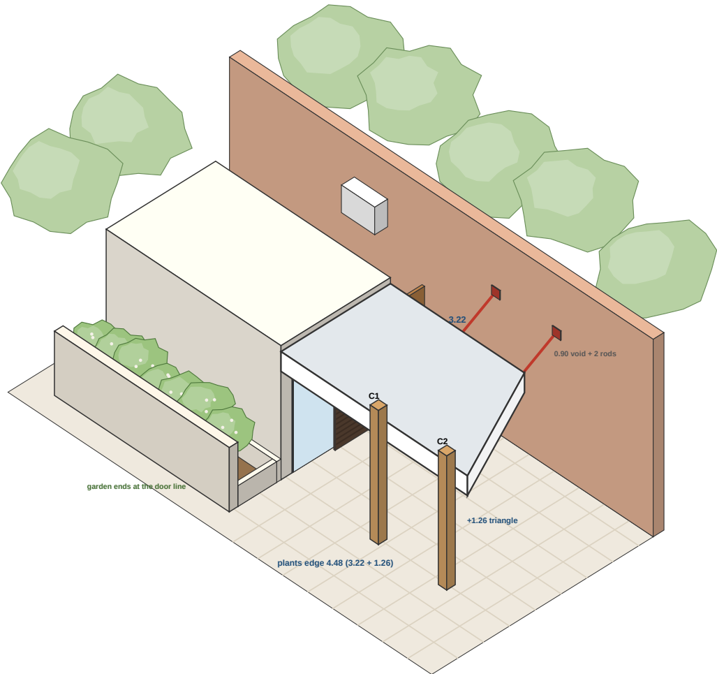
4/V2T-02 3D VIEW — from the plants side (courtyard)
