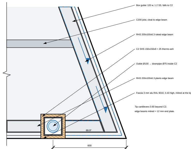
D3 TIP AT C2 (triangle) — PLAN 1:15
