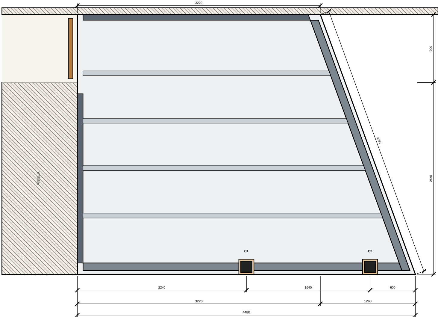
1 TOP VIEW — ANNEX, GARDEN & ROOF V1T-01 1:50 @ A3 garden ends at the door line; trees = background
