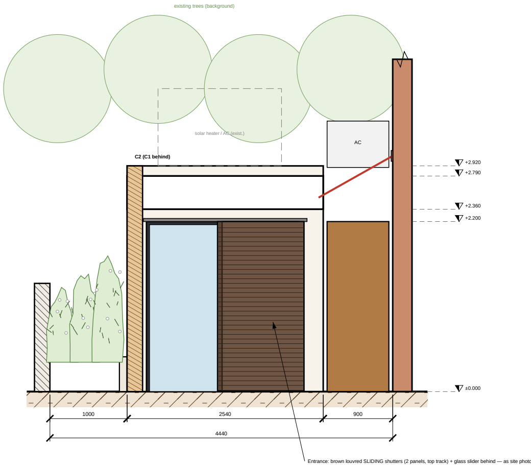
2/V2-02 PLANTS-SIDE ELEVATION — C1 + C2 — 1:50
