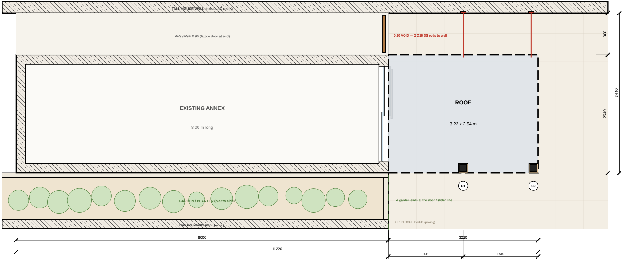
1 TOP VIEW — ANNEX, GARDEN & ROOF V2-01 1:50 @ A3 garden ends at the door line; trees = background
