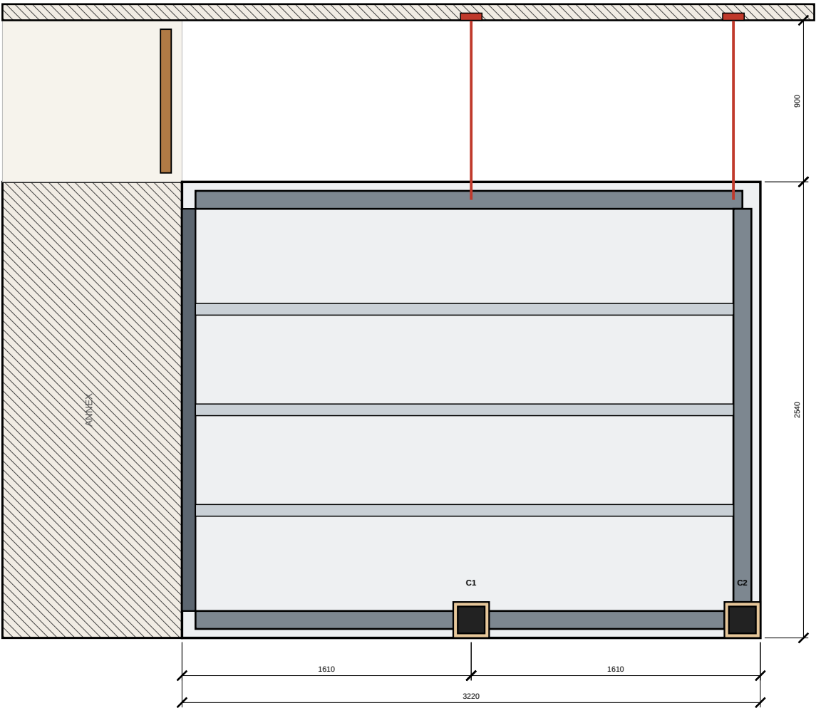
1 TOP VIEW — ANNEX, GARDEN & ROOF V2-01 1:50 @ A3 garden ends at the door line; trees = background
