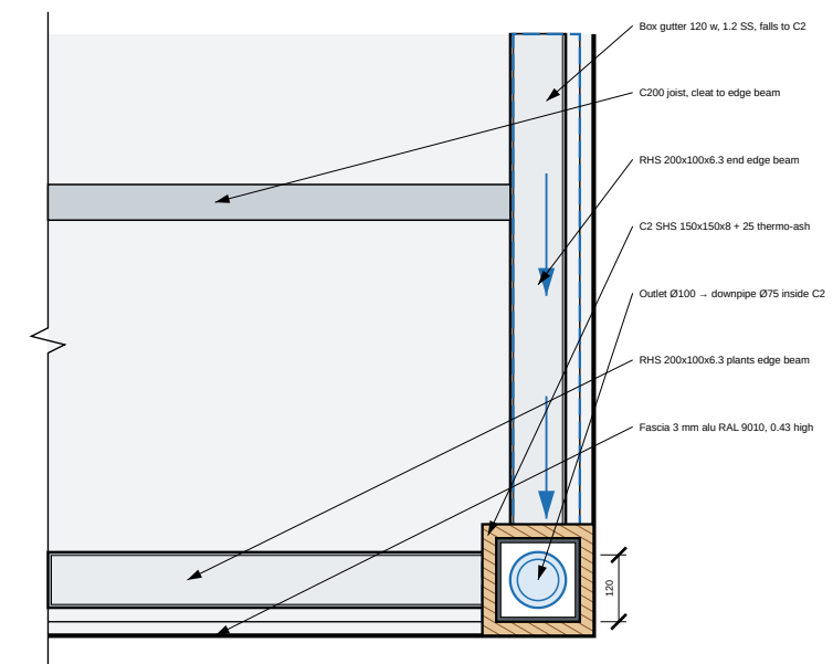
D3 CORNER AT C2 — PLAN 1:15
