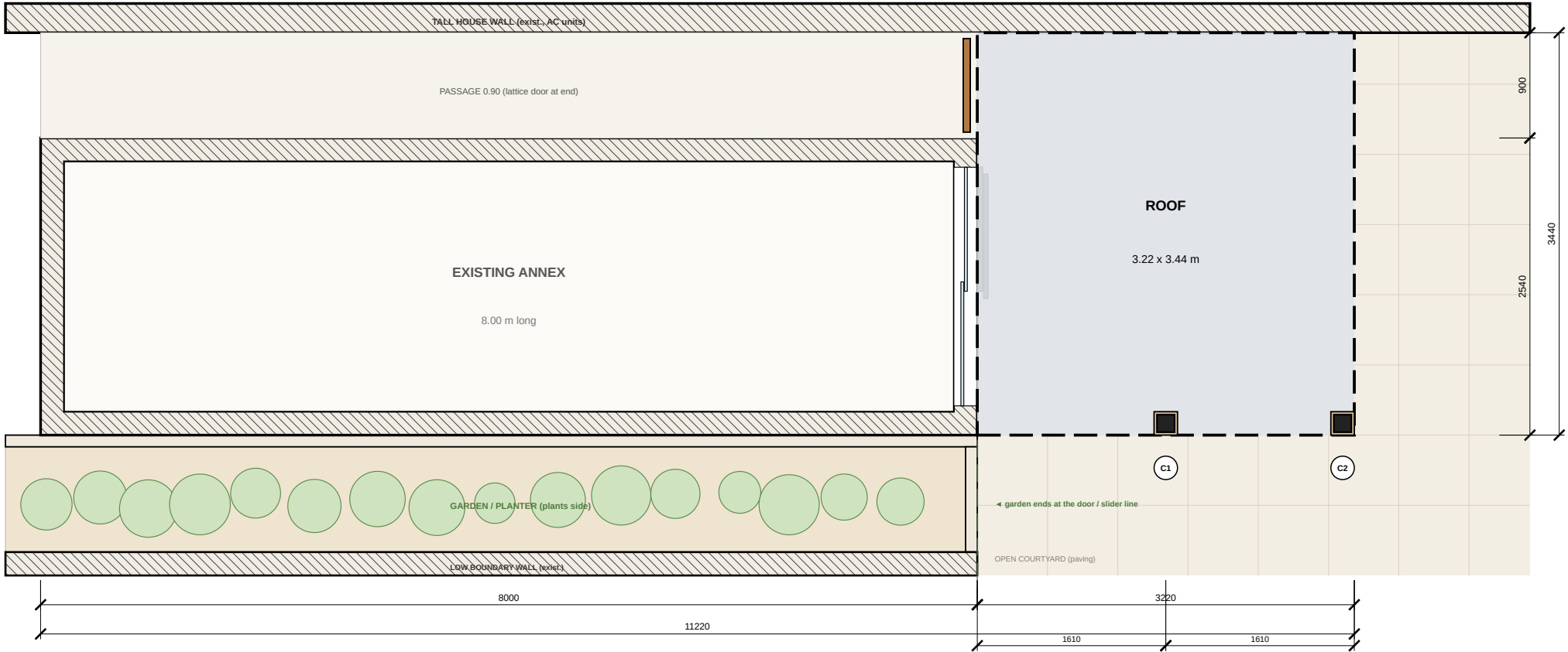
1 TOP VIEW — ANNEX, GARDEN & ROOF V1-01 1:50 @ A3 garden ends at the door line; trees = background
