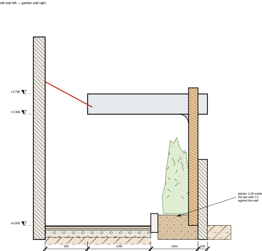
3/V2T-02 SECTION ACROSS AT C1 — 1:50 (refined: V2T-03)
