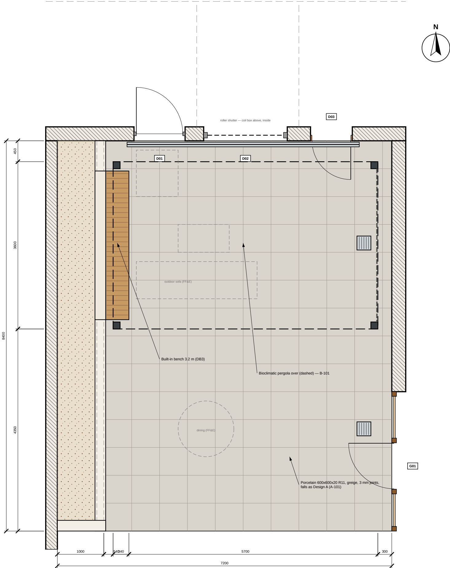
1 GENERAL ARRANGEMENT PLAN B-100 1:50 @ A3
