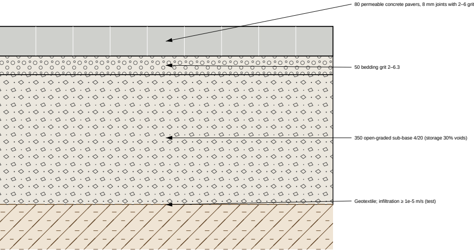
DD3 PERMEABLE PAVING (SuDS) — 1:10
