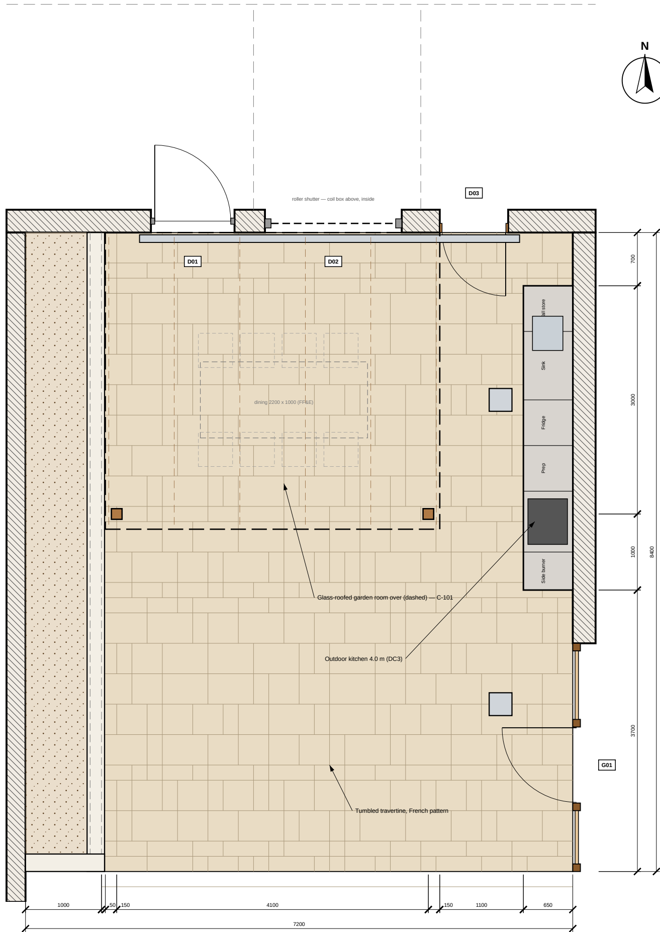
1 C-100 GENERAL ARRANGEMENT PLAN 1:50 @ A3
