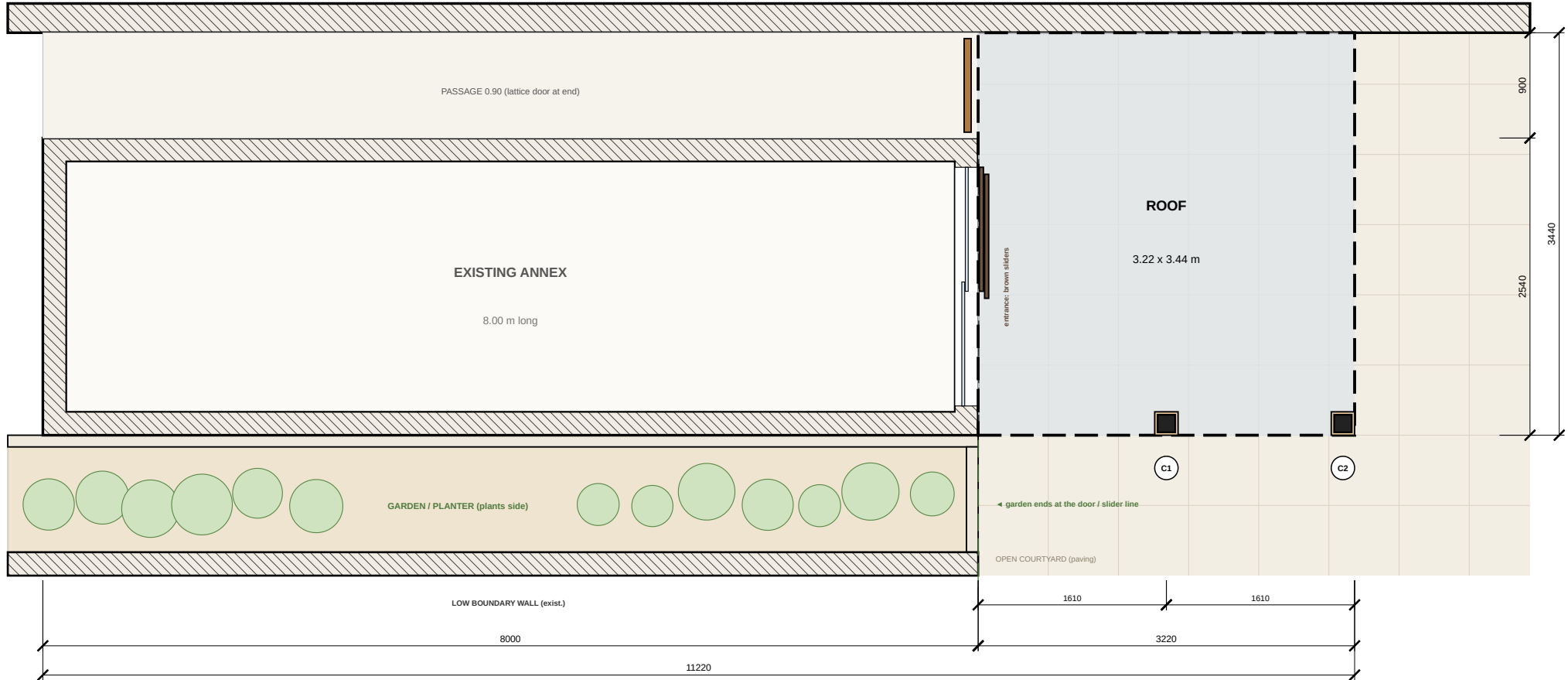
1 TOP VIEW — ANNEX, GARDEN & ROOF V1-01 1:50 @ A3 — garden ends at the door line; trees = background
