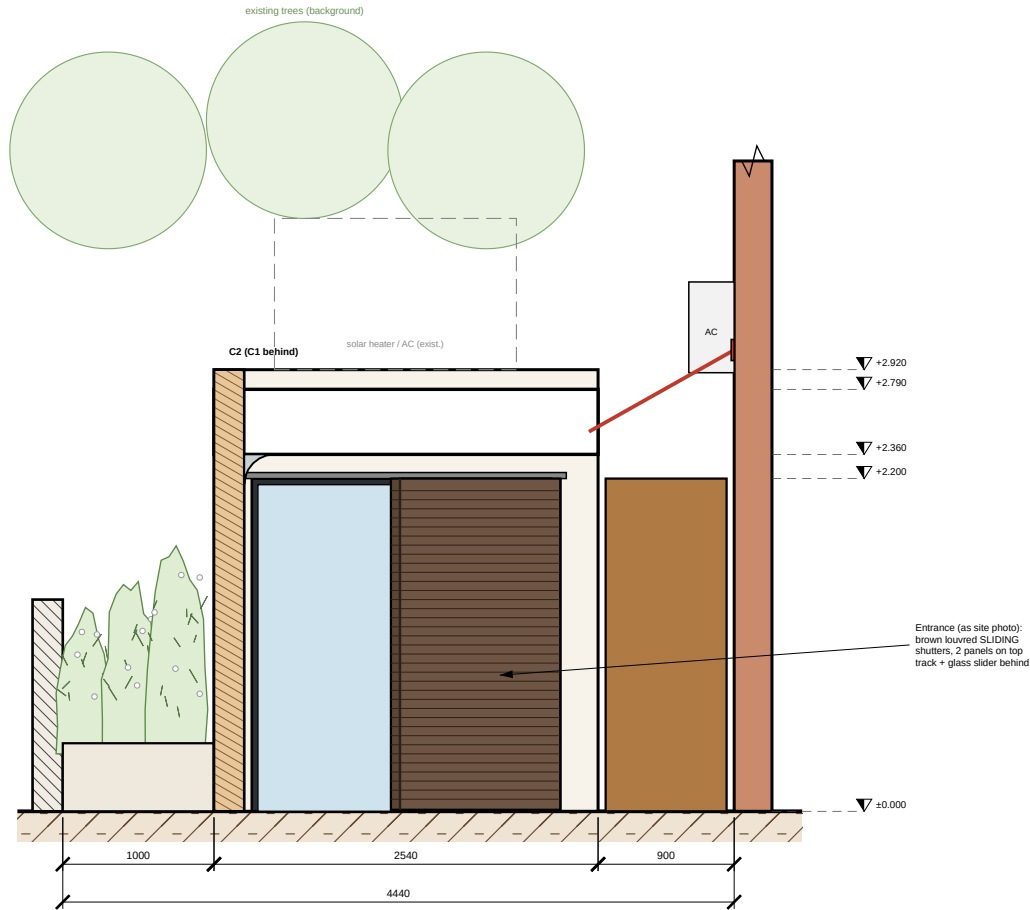
1/V2-02 VIEW TO ANNEX FAÇADE (as site photo) — 1:50
