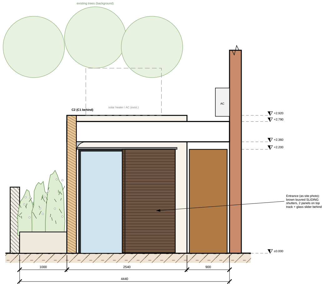
1/V1-02 VIEW TO ANNEX FAÇADE (as site photo) — 1:50
