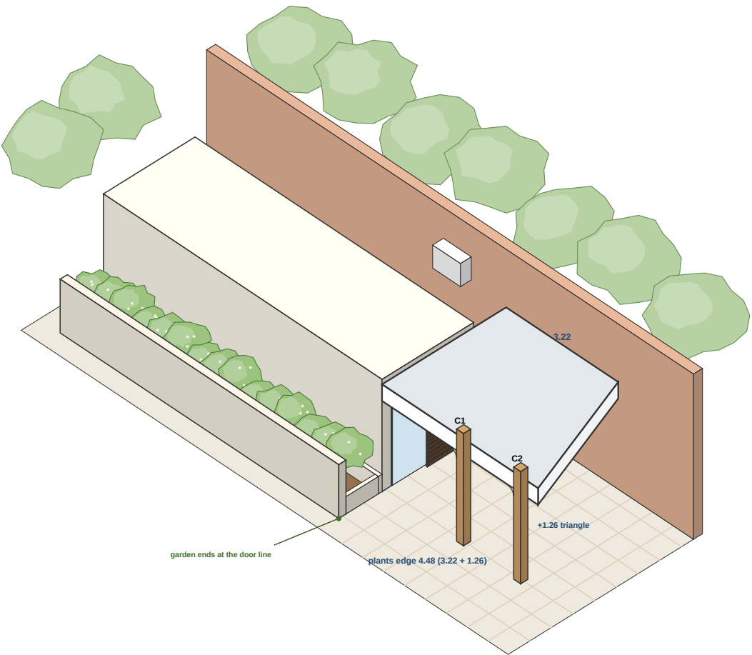
4/V1T-02 3D VIEW — from the plants side (courtyard)
