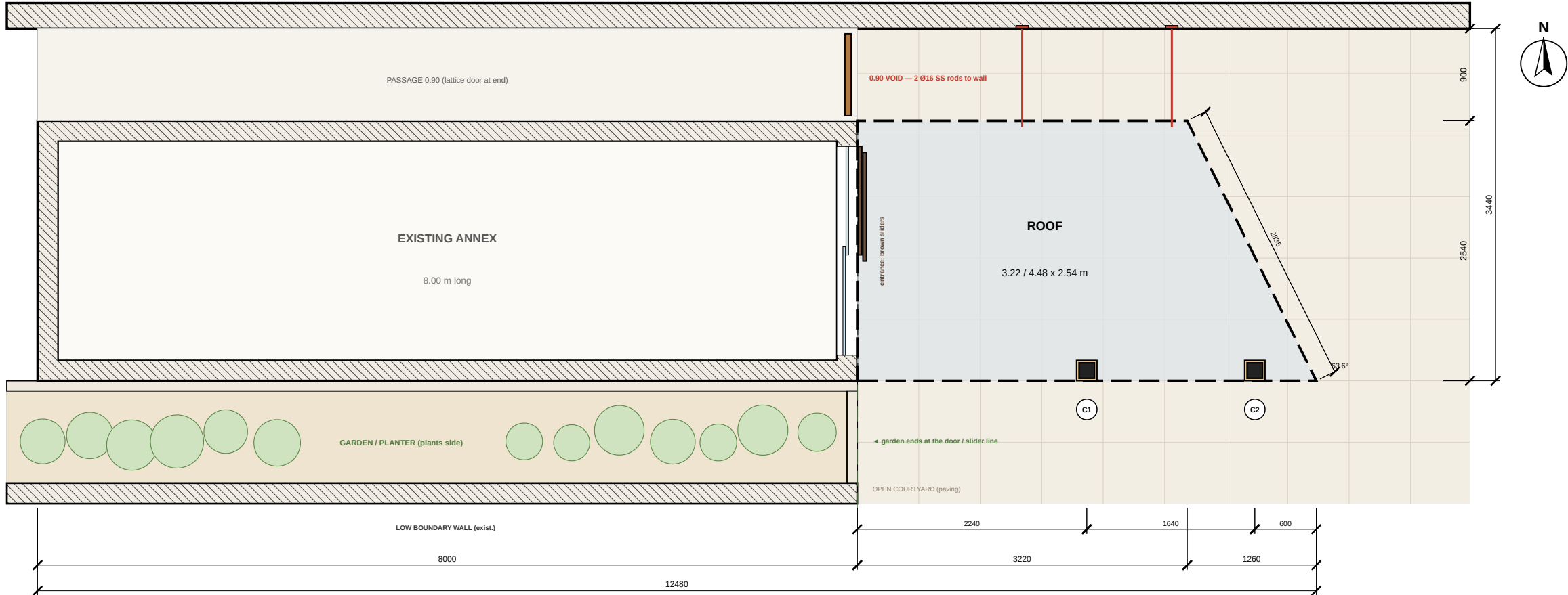
1 TOP VIEW — ANNEX, GARDEN & ROOF V2T-01 1:50 @ A3 — garden ends at the door line; trees = background
