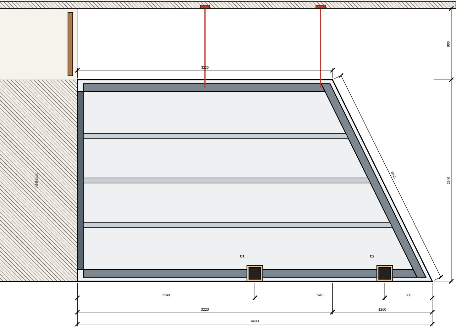
1 TOP VIEW — ANNEX, GARDEN & ROOF V2T-01 1:50 @ A3 — garden ends at the door line; trees = background
