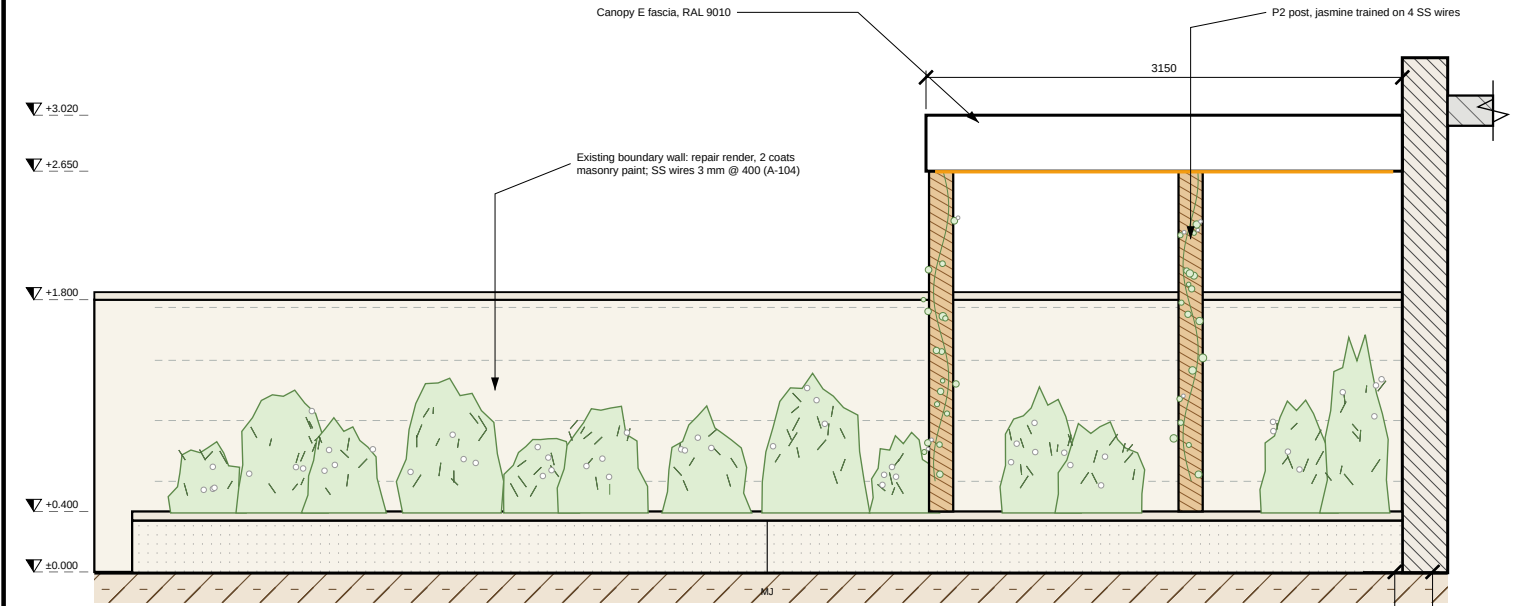
1 ELEVATION B — PLANTER & BOUNDARY WALL (looking west) A-201 1:50 @ A3
