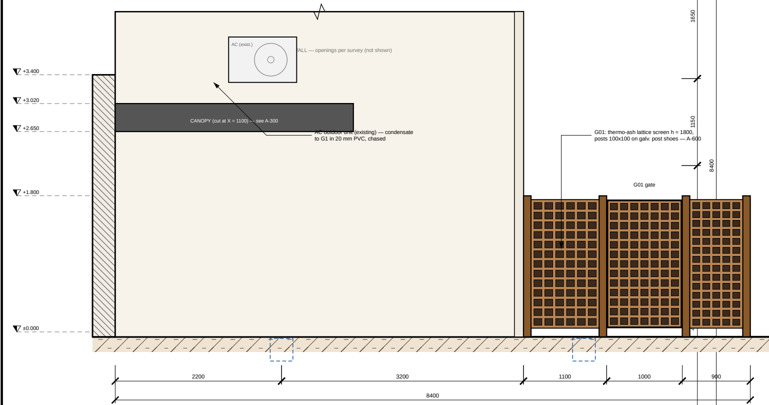
2 ELEVATION C — HOUSE WALL & SCREEN (looking east) A-201 1:50 @ A3
