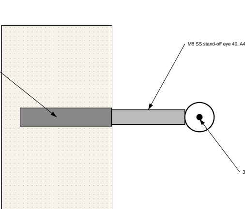
D8 CLIMBING WIRE FIXING — 1:2
