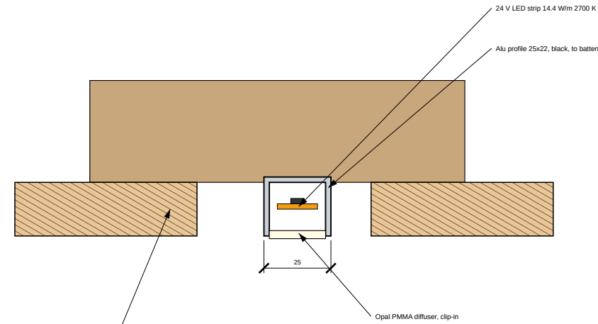
D5 LED PROFILE IN SOFFIT — 1:2
