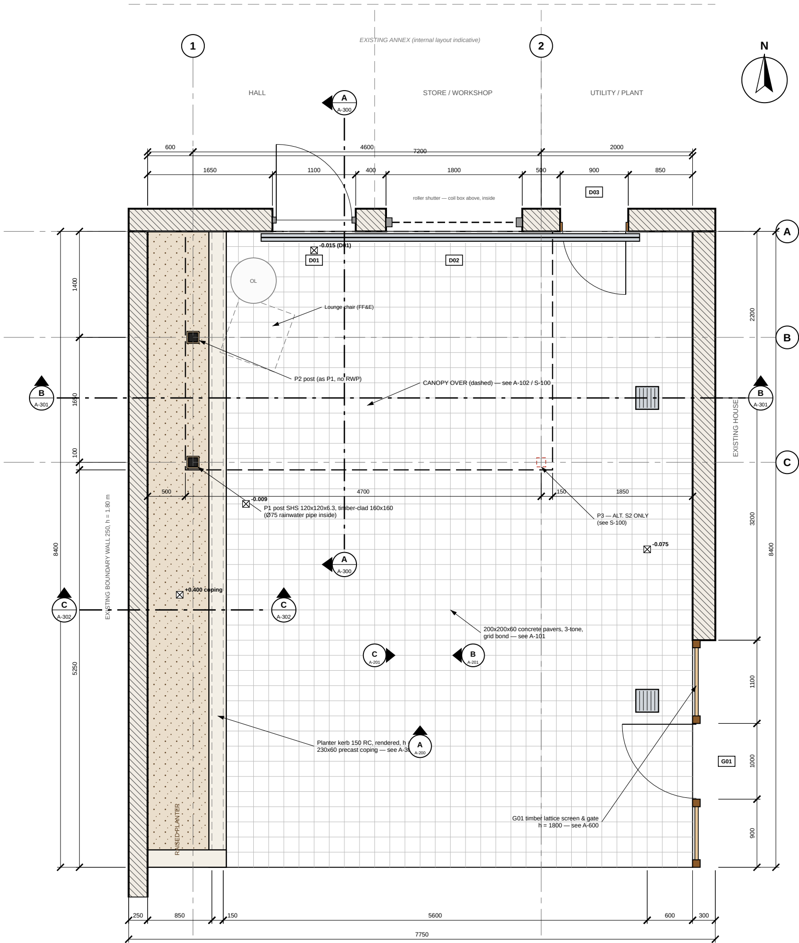
1 A-100 COURTYARD GENERAL ARRANGEMENT PLAN 1:50 @ A3 cut plane +1.20
