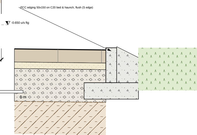
4/A-302 SOUTH EDGE RESTRAINT — 1:10
