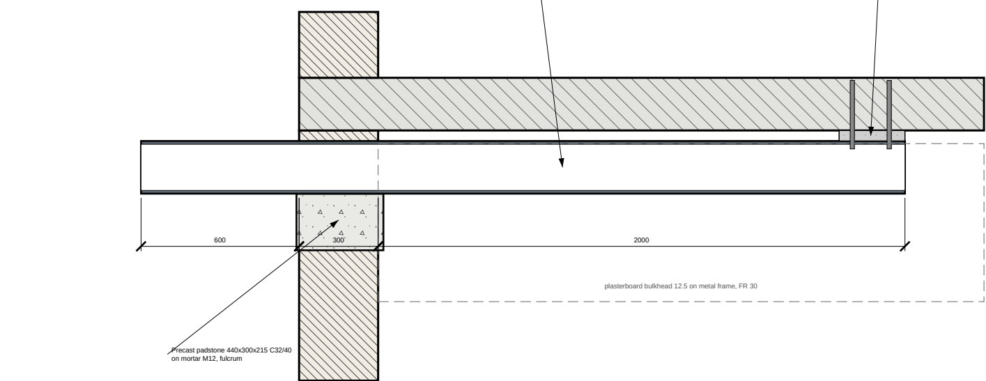
D7 B2 BACK-SPAN (SCHEME S1) — 1:20
