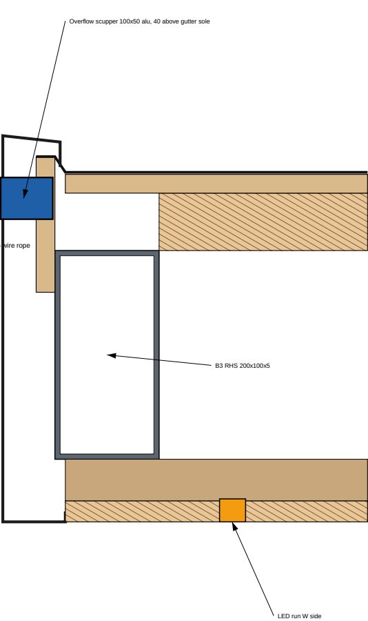
D9 WEST FASCIA & OVERFLOW — 1:5
