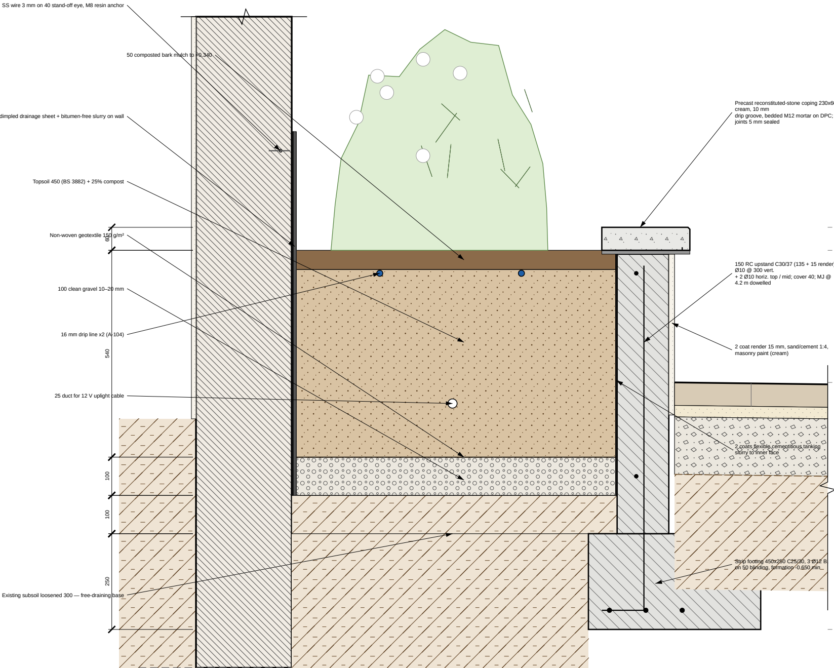
1 SECTION C-C — RAISED PLANTER 1:10 @ A3 at Y = -5000, looking north
